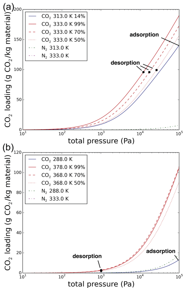
Fig. 8 The \text{CO}_2 and \text{N}_2 isotherms of NaX for carbon capture from coal-fired power plant flue gases (a) and direct air capture (b), respectively. The adsorption and different desorption conditions indicated are depending on the imposed purity of the \text{CO}_2 .
