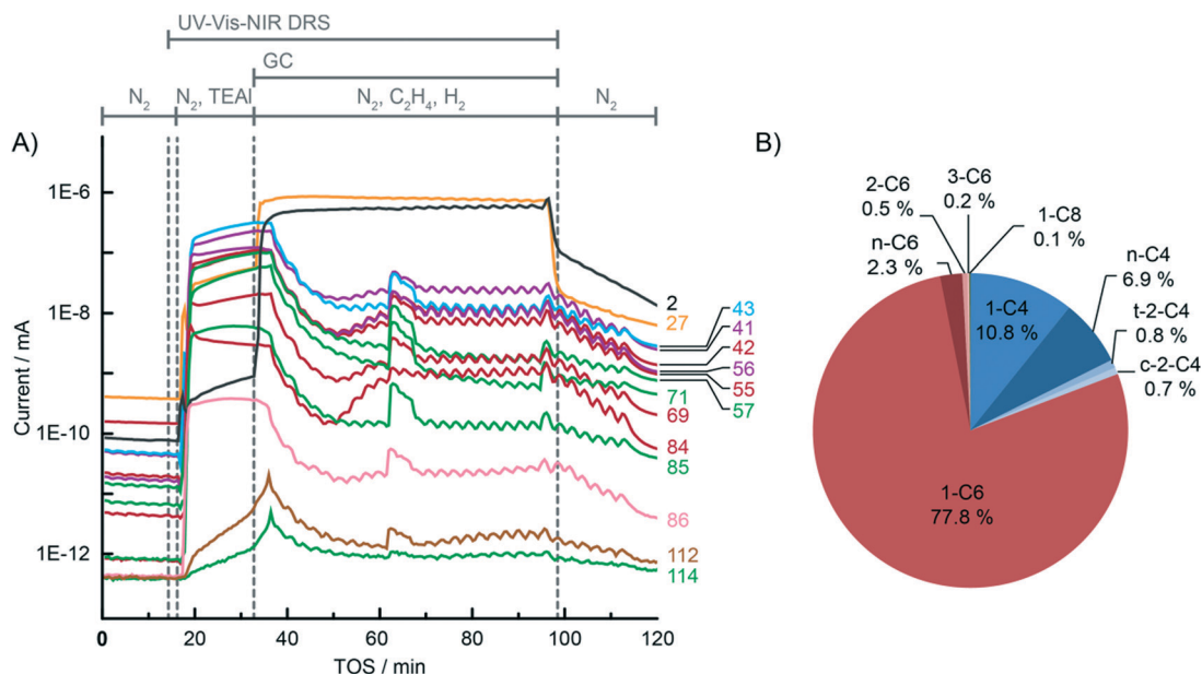
Fig. 2 A) On-line MS analysis of the gas phase during the modification of the CS Phillips-type Cr/SiO 2 catalyst with the TEAL co-catalyst and subsequent oligo-/polymerisation of ethylene using the in-house designed operando setup. UV-vis-NIR DRS repeated measurements were started at t = 14 min. At t = 16 min, TEAL was injected into the system via evaporation into the N 2 stream. After 17 min, the gas feed was changed to the reaction mixture consisting of 45% N 2 , 45% C 2 H 4 and 10% H 2 , at a total flow rate of 10 cm 3 min -1 and the gas phase was sampled for the GC analysis. After 60 min of reaction, the gas feed was changed back to N 2 and UV-vis-NIR DRS and GC sampling stopped. Assignment of the m/z is as follows: 2 H 2 ; 27 ethylene, 1-butene, 1-hexene, hexane, TEAL, butane, heptanes; 43 1-butene, butane, heptanes, octane; 41 1-butene, 1-hexene, hexane, butane, heptanes; 56 1-hexene, hexane, 1-butene; 42, 55, 69, 84 1-hexene, 1-octene; 57 hexane, TEAL, heptanes; 71, 85 TEAL, octane; 71, 85, 114 TEAL; 86 hexane and 112 1-octene. B) GC analysis of the gas phase collected during oligo-/polymerisation of ethylene after the modification of the catalyst with TEAL.
