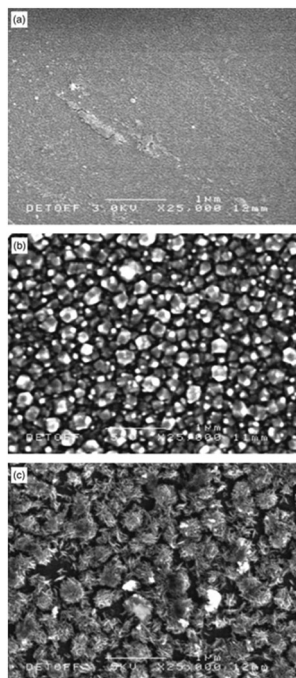
Fig. 24 SEM of films grown from AACVD deposition of InMe 3 and MeOH at (a) 400 °C; (b) 450 °C; and (c) 500 °C. Reproduced with permission from ref. 176 Copyright 2013 Royal Australian Chemical Institute.
