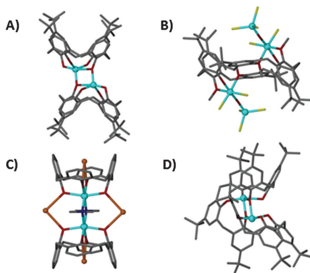
Fig. 1 Examples of Ti(IV) calix[ n ]arene complexes from Power, Atwood, Raston and Pedersen (A–D respectively). Clockwise from top left: \text{Ti}_2\text{TBC}[4]_2 (A), \text{Ti}_4\text{TBC}[6]\text{Cl}_{10} (B), \text{Ti}_2\text{Na}_2\text{C}[4]_2 (C), [\text{Ti}_2\text{TBC}[8](\text{O}^i\text{Pr})_2]^- (D). Colour code: C = grey, O = red, Ti = blue, Cl = yellow, Na = orange. H-atoms omitted for clarity.
