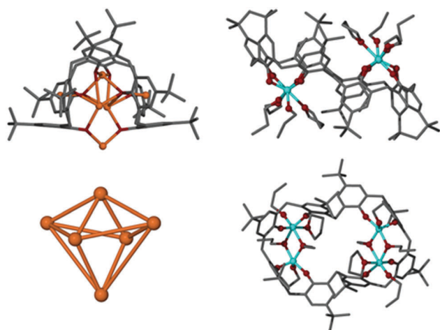
Fig. 2 Top left: \text{Na}_6\text{TBC}[8](\text{THF})_7 (1) complex and below, the \text{Na}_6 metallic core. Top right: \text{Ti}_4\text{TBC}[8](\text{O}^i\text{Pr})_8(\text{THF})_2 (2) and below, the orthogonal view. Colour code: C = grey, O = red, Ti = blue, Na = orange. H-atoms omitted for clarity.
