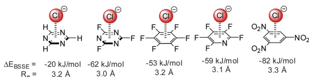
Fig. 2 Interaction energy with basis set superposition error correction ( E_{\text{BSSSE}} ) and equilibrium distances ( R_{\text{a}} ) of selected anion- \pi complexes from the MP2/6-31++G** level of theory. 7,15,16
