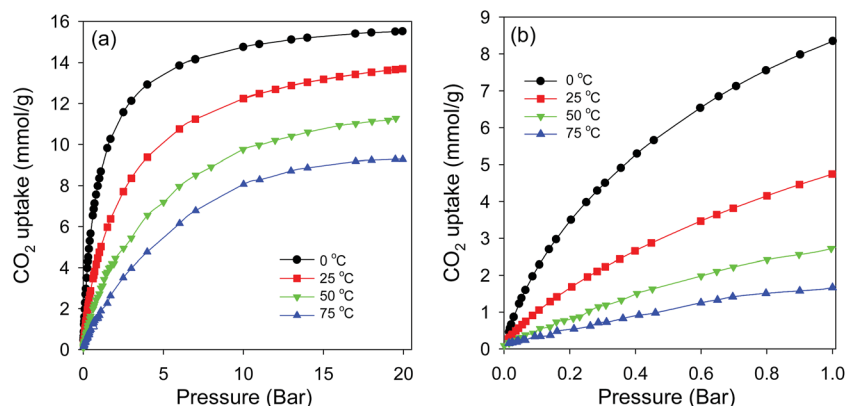
Fig. 11 \text{CO}_2 uptake isotherms for sample CN2650 at various temperatures; (a) 0 – 20\text{ bar} , (b) low pressure ( 0 – 1\text{ bar} ).
