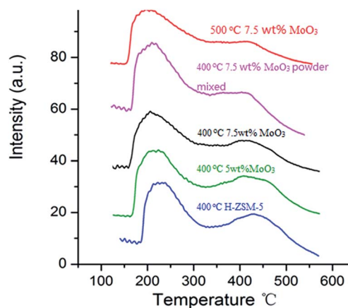
Fig. 6 \text{NH}_3 -temperature programmed desorption profiles of \text{MoO}_3/\text{H-ZSM-5} samples prepared via different conditions (impregnation/powder mixing, 400\text{--}500\text{ }^\circ\text{C} ) together with the original H-ZSM-5 sample ( 400\text{ }^\circ\text{C} ).
