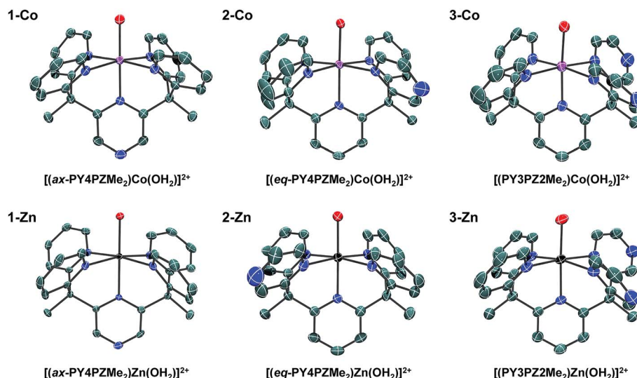
Fig. 2 Crystal structures of cations in the following salts: 1-Co , [(ax-PY4PZMe_2)Co(OH_2)](OTf)_2 ; 2-Co , [(eq-PY4PZMe_2)Co(OH_2)](OTf)_2 ; 3-Co , [(PY3PZ2Me_2)Co(OH_2)](OTf)_2 ; 1-Zn , [(ax-PY4PZMe_2)Zn(OH_2)](OTf)_2 ; 2-Zn , [(eq-PY4PZMe_2)Zn(OH_2)](OTf)_2 ; 3-Zn , [(PY3PZ2Me_2)Zn(OH_2)](OTf)_2 . Thermal ellipsoids are drawn at the 70% probability level. Hydrogen atoms have been omitted for clarity.
