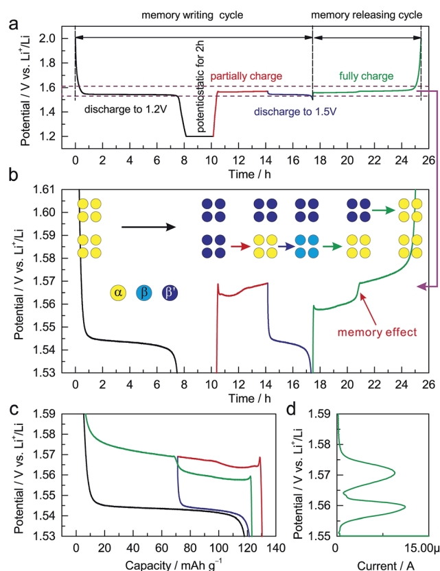
Fig. 4 Demonstration of a memory effect in Al-doped \text{Li}_4\text{Ti}_5\text{O}_{12} (ALTO). (a) Memory-writing cycle: discharge to 1.2 V and potentiostatic for 2 h (black), partially charge for 4 h (red), and discharge to 1.5 V (blue); memory-releasing cycle: full charge to 2.0 V (green). The current rate is 0.1 C. (b) Enlarged view between 1.53 and 1.61 V. The inset shows the corresponding phase transition, in which \alpha is the delithiated phase, \beta is the lithiated phase discharged to 1.5 V, and \beta' is the lithiated phase discharged to 1.2 V and potentiostatic for 2 h. (c) The charge/discharge curves in these memory-writing/releasing cycles. (d) The linear sweep voltammetry (LSV) curve of ALTO with a scan rate of 1 \mu\text{V s}^{-1} from 1.55 to 1.59 V after the same memory-writing cycle.
