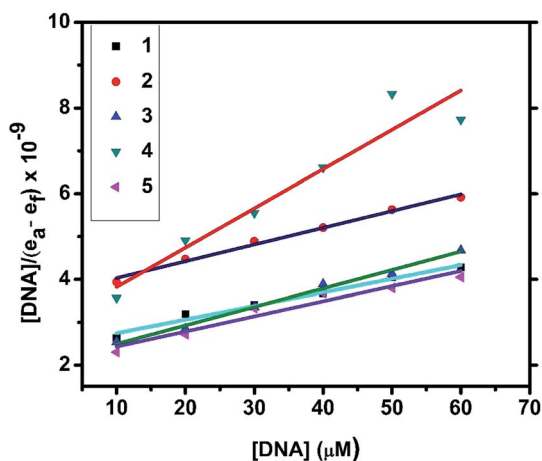
Fig. 7 Plots of [DNA]/(\epsilon_a - \epsilon_f) versus [DNA] for the titration of the complexes with CT DNA.
