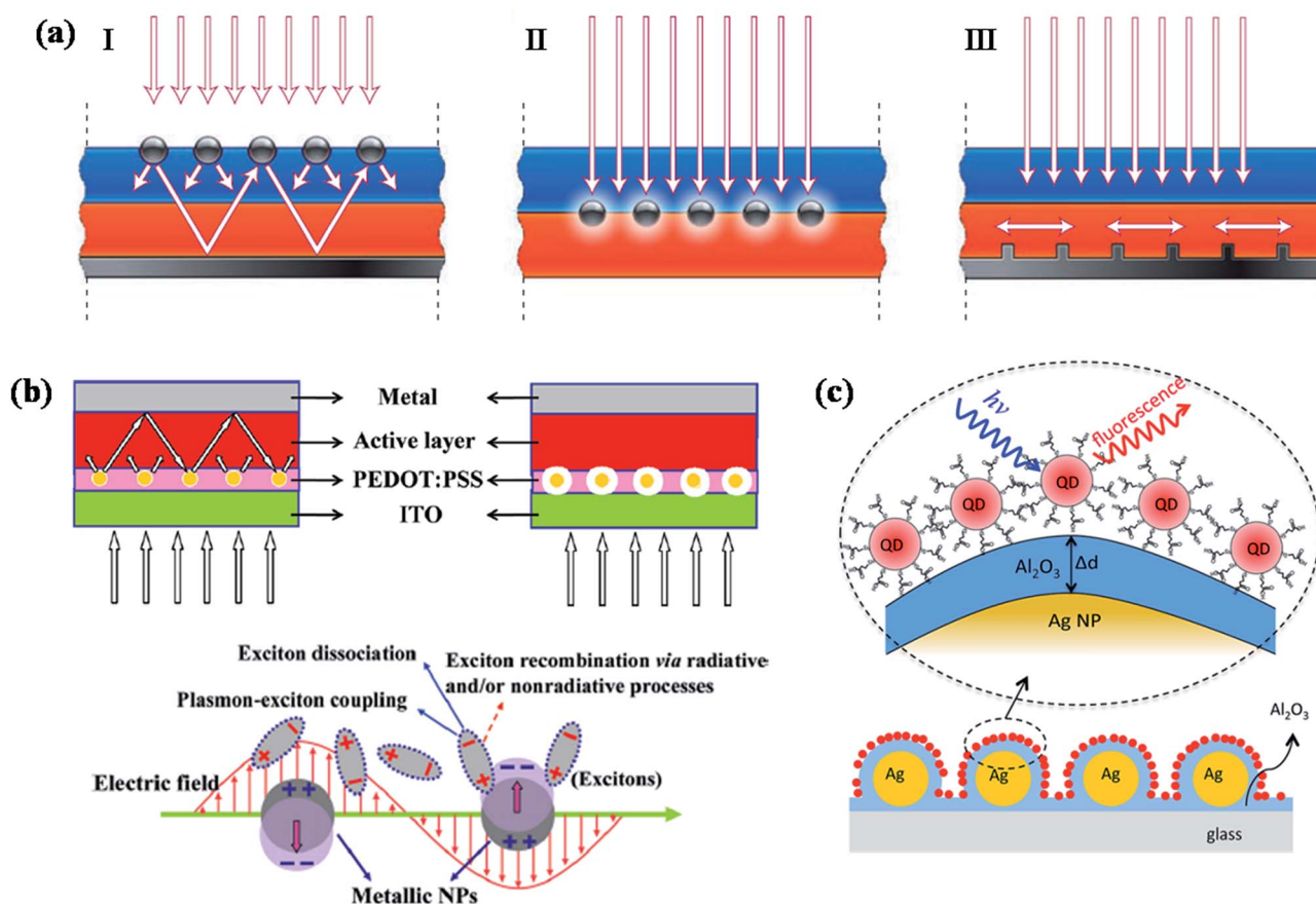
Fig. 13 (a) Schematic showing different design strategies for light trapping in solar cells. Light can be trapped via (I) multiple light scattering (II), (III) LSPR induced field enhancement, and (III) by the excitation of surface plasmon polaritons at the metal/semiconductor interface. (b) Schematic representation plasmonic bulk heterojunction (BHJ) solar cell, in which plasmonic NPs are embedded in PEDOT:PSS layer. The optical path length increased because of multiple and high-angle scattering light scattering in active layer in the presence of plasmonic NPs (left). In addition to light scattering, electric field enhancement also contributes to the enhanced efficiency (right). Schematic representation showing the exciton–plasmon coupling led to enhancement in rate of exciton dissociation, thereby reducing exciton recombination. (c) Schematic illustration of CdSe NPs on Al 2 O 3 -coated Ag NPs surface. The distance between Ag NP film and CdSe NPs are tuned by varying the thickness of the Al 2 O 3 layer. Optical properties (fluorescence and fluorescence life time) of QDs as a function of distance between QDs and Ag film are recorded to investigate the distance dependent plasmonic effect of Ag NPs. Figures (a), (b) and (c) reproduced with permission from ref. 44, 148 and 178, respectively.
