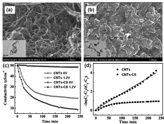
Fig. 23 SEM images of (a) CNTs and (b) CNTs–CS. The insets are their TEM images. (c) Variation of solution conductivity with time and (d) linear plot of the pseudo-first-order kinetic equation for the electro-sorption of \text{Cu}^{2+} by CNTs and CNTs–CS. (Reproduced with permission from ref. 59.)
