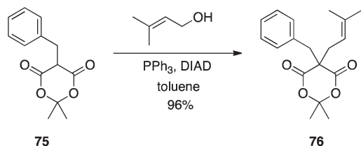
Scheme 23 C-alkylation of C 5 -mono-substituted Meldrum's acids.
