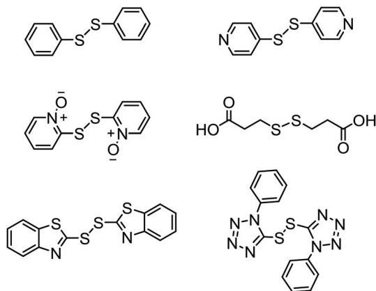
Chart 3 Thiol and disulfide compounds used as co-initiators in photo-induced free radical polymerization in the presence of thioxanones.
