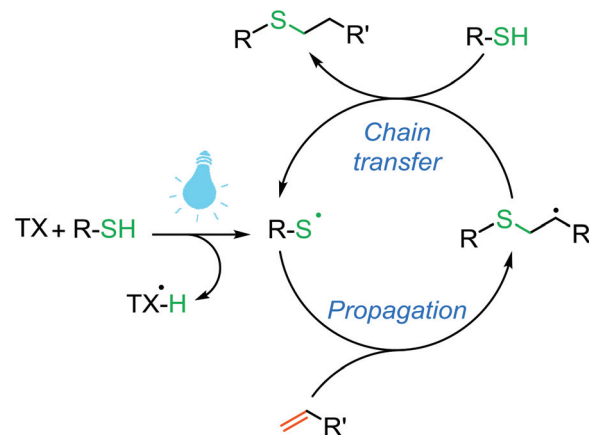
Scheme 7 Light-induced thiol-ene click reaction.
