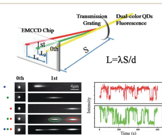
Fig. 4 Multicolour super-resolution of three different QDs with PL maxima at 525 nm (blue), 585 nm (green), and 655 nm (red) separated by DNA at distances below 50 nm. Top: a transmission grating is used for colour separation (dual colour experiment is shown). Bottom left: zero and first order images of single QDs and combinations of two and three QDs. Bottom right: taking the first order images the blinking behaviour of the green and red QD can be distinguished for super-resolution imaging. Reproduced with permission from ref. 133. Copyright 2012 American Chemical Society.
