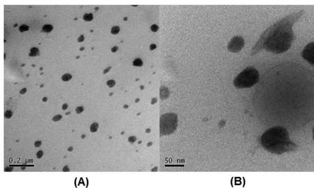
Fig. 2 TEM image of M3 micelles (loaded with curc and crosslinked with Pt) (concentration of micelles 1 \text{ mg mL}^{-1} in water): A (scale bar = 200 nm) and B (scale bar = 50 nm).
