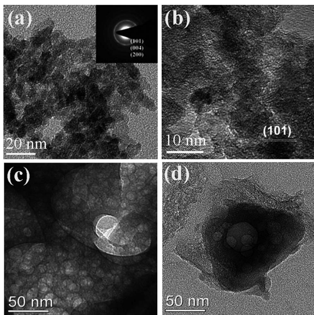
Fig. 6 (a) TEM image and (b) HRTEM image of \text{TiO}_2 with wormhole mesopores. 98 (c and d) TEM images of porous \text{Li}_3\text{V}_2(\text{PO}_4)_3/\text{C} . 61 Adopted from ref. 61, Copyright 2012, with permission from Elsevier.
