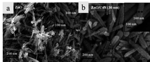
Fig. 7 FESEM images of (a) ZnO nanorods and (b) CdS/ZnO nanorods (reprinted with permission from ref. 67, copyright 2012 American Chemical Society).
