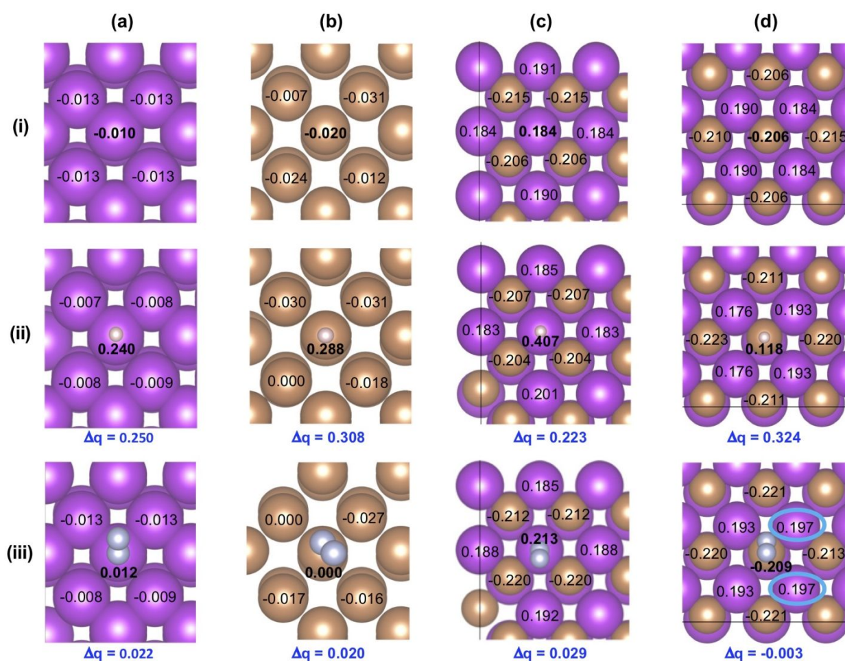
Figure 7. Bader charge analysis of (a) Bi, (b) Sb, (c) Bi in BiSb, and (d) Sb in BiSb on their (012) planes; (i) the pristine surface, (ii) the surface when H is adsorbed and (iii) the surface when N_2 is adsorbed (Bi: violet, Sb: golden, N: gray, and H: beige). The atomic charges are indicated on the corresponding atoms. \Delta q represents the change in charge at the binding site after H or N_2 adsorption. In (d-iii), the blue circles represent charges on Bi atoms that changed considerably by N_2 adsorption on Sb.
