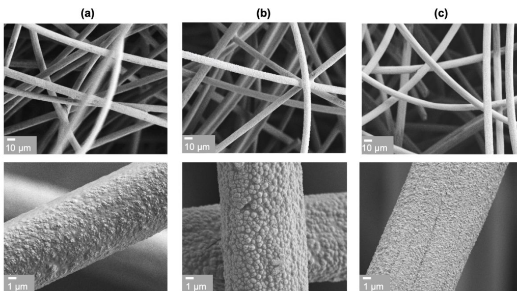
Figure 1. SEM images of (a) Bi, (b) Sb, and (c) BiSb deposited on the carbon felt substrate. The bottom panels show corresponding higher-magnification images of Bi, Sb, and BiSb deposits on a single carbon fiber.
