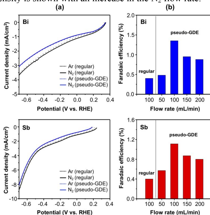
Figure 3. (a) LSVs of Bi (top) and Sb (bottom) as a regular electrode (black) and as a pseudo-GDE (blue) in 0.5 M borate (pH 9.3) with Ar (dotted) or ^{15}\text{N}_2 (solid) (scan rate, 25 mV/s). The gas flow rate was 100 mL/min for all cases. (b) FEs for ^{15}\text{NH}_3 of Bi (top) and Sb (bottom) as a regular electrode and as a pseudo-GDE with various ^{15}\text{N}_2 flow rates at -0.6 V vs RHE.
