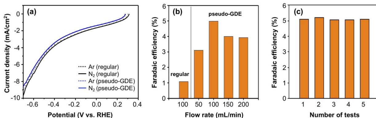
Figure 4. (a) LSVs of BiSb as a regular electrode (black) and as a pseudo-GDE (blue) in 0.5 M borate (pH 9.3) with Ar (dotted) or ^{15}\text{N}_2 (solid) (scan rate, 25 mV/s). The gas flow rate was 100 mL/min. (b) FEs for ^{15}\text{NH}_3 of BiSb as a regular electrode and as a pseudo-GDE with various ^{15}\text{N}_2 flow rates at -0.6 V vs RHE. (c) FEs for ^{15}\text{NH}_3 of BiSb as a pseudo-GDE with the \text{N}_2 flow rate of 100 mL/min at -0.6 V vs RHE for five consecutive experiments.
