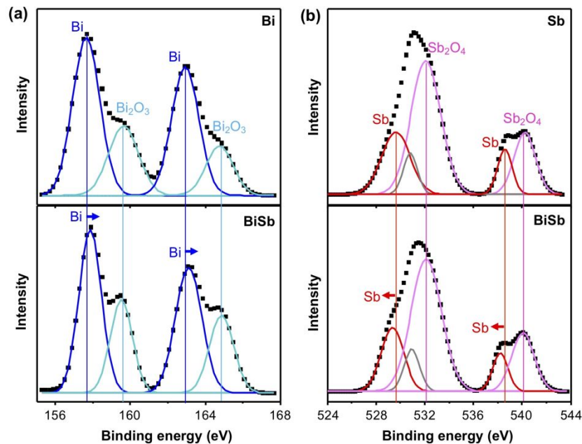
Figure 6. XPS spectra of the (a) Bi 4f region of Bi (top) and BiSb (bottom) and (b) Sb 3d region of Sb (top) and BiSb (bottom) (black squares: experimental data, blue line: Bi metal peak, light blue line: \text{Bi}_2\text{O}_3 peak, red line: Sb metal peak, pink line: \text{Sb}_2\text{O}_4 peak, gray line: oxygen 1s peak).
