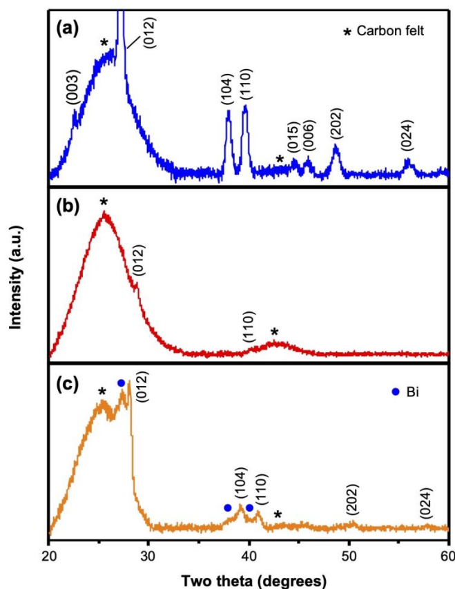
Figure 2. XRD patterns of as-deposited (a) Bi, (b) Sb, and (c) BiSb on carbon felt. The (hkl) indices are assigned from the PDF cards for Bi (44-1246) and Sb (35-0732). The broad peaks corresponding to the carbon felt are denoted by an asterisk. Bi (R -3 m, a = 0.454650 nm and c = 1.186294 nm), Sb (R -3 m, a = 0.430777 nm and c = 1.127662 nm) and BiSb (R -3 m, a = 0.442680 nm and c = 1.160351 nm). 36
