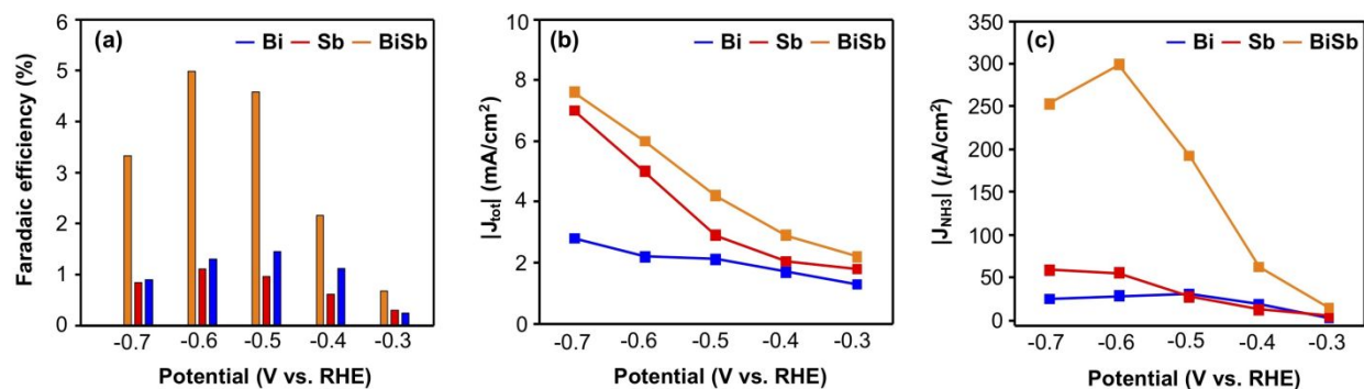
Figure 5. (a) FEs for NH_3 , (b) total current densities, and (c) partial current densities associated with ^{15}NH_3 production by Bi, Sb, and BiSb pseudo-GDE electrodes with the N_2 flow rate of 100 mL/min in 0.5 M borate (pH 9.3).
