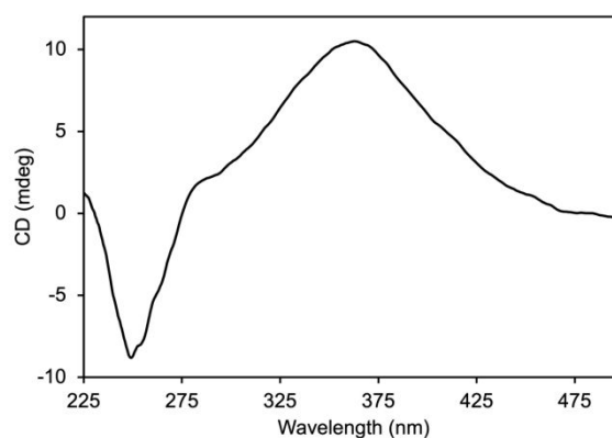
Figure 5. CD spectrum of co-PIC-brush-Pd-Pin-PS . (DCE, 25 ^\circ\text{C} )
