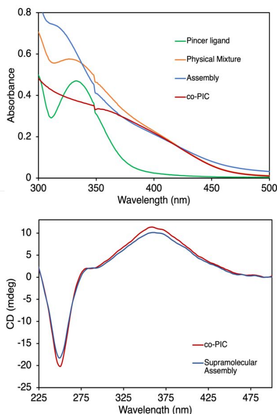
Figure 3. Spectroscopic analysis of co -PIC assembly with \text{Pd} -Pin. (top) UV-Vis traces of (green) \text{Pd} -Pin, (red) co -PIC, (orange) physical mixture, and (blue) metal coordination after \text{AgBF}_4 addition, recorded in DCE at 25 °C with [\text{co-PIC}] = 7.5 \mu\text{M} . (bottom) CD traces of (red) co -PIC and (blue) metal coordination after \text{AgBF}_4 addition, recorded in DCE at 25 °C with [\text{co-PIC}] = 7.5 \mu\text{M} .
