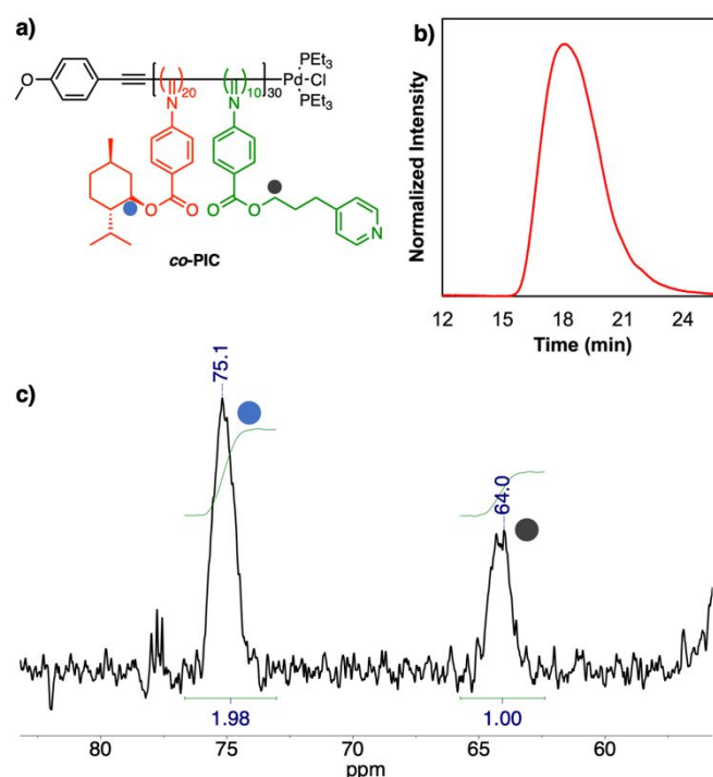
Figure 1. (a) Structure of the side-chain functionalized helical co -PIC with dots highlighting backbone signals of interest in the 13 C NMR spectrum. (b) SEC curve of co -PIC showing number average molecular weight ( M n ) of 7,200 and dispersity ( D ) of 1.44. (c) Partial 13 C NMR spectrum (600 MHz, CD 2 Cl 2 ) of co -PIC showing backbone signals from two types of monomers. Integration of these signals confirms that the ratio of chiral to achiral component is 2:1.
