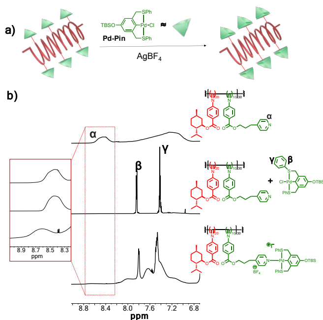
Figure 2. (a) Schematic representation of the side-chain supramolecular assembly of co -PIC and \text{Pd} -Pin complex. (b) Partial ^1\text{H} NMR (600 MHz) spectroscopic overlay of (top to bottom) co -PIC, physical mixture of co -PIC and \text{Pd} -Pin, and metal coordination assembly after \text{AgBF}_4 addition.
