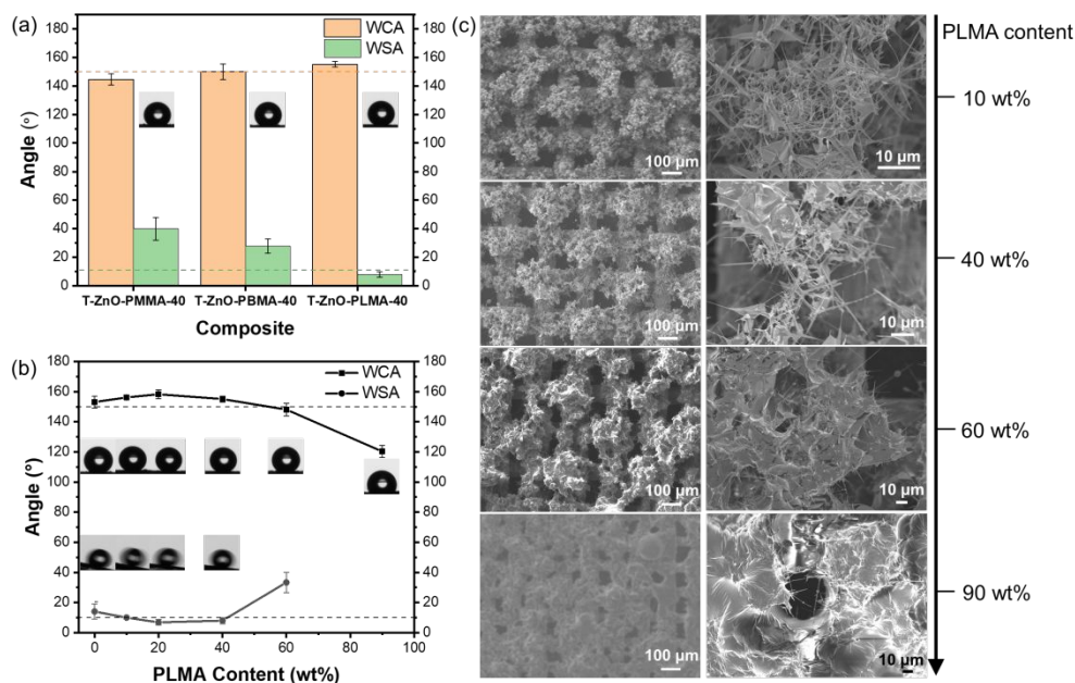
Figure 2. Wettability of T-ZnO/polymer hybrid meshes with different (a) polymers and (b) PLMA content; (c) SEM images of T-ZnO/polymer hybrid meshes with different PLMA content.
