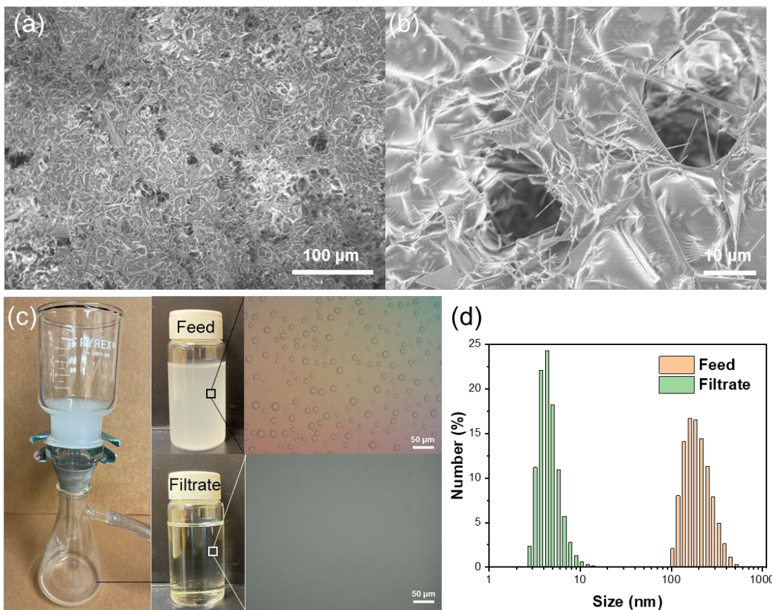
Figure 5. (a), (b) SEM images of a T-ZnO/PLMA coated quantitative filter paper. (c) Photographic and optical microscopy images of a surfactant-stabilized water-in-hexane emulsion before and after being filtered through the T-ZnO/PLMA coated filter paper. (d) Normalized water size distribution of the feed and filtrate measured by dynamic light scattering.
