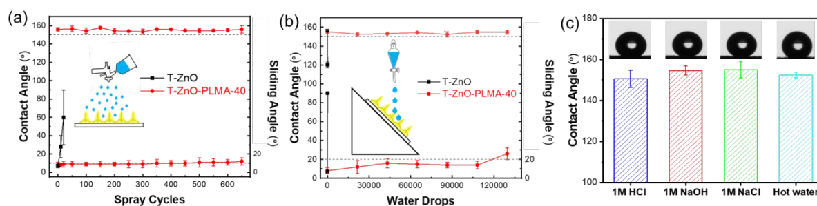
Figure 6. The durability of T-ZnO coated mesh and T-ZnO/PLMA-40 against (a) water spray impact and (b) water droplet impact. (c) Contact angles of strong acid, base, salt solution, and 70^\circ\text{C} water droplets on T-ZnO/PLMA-40.
