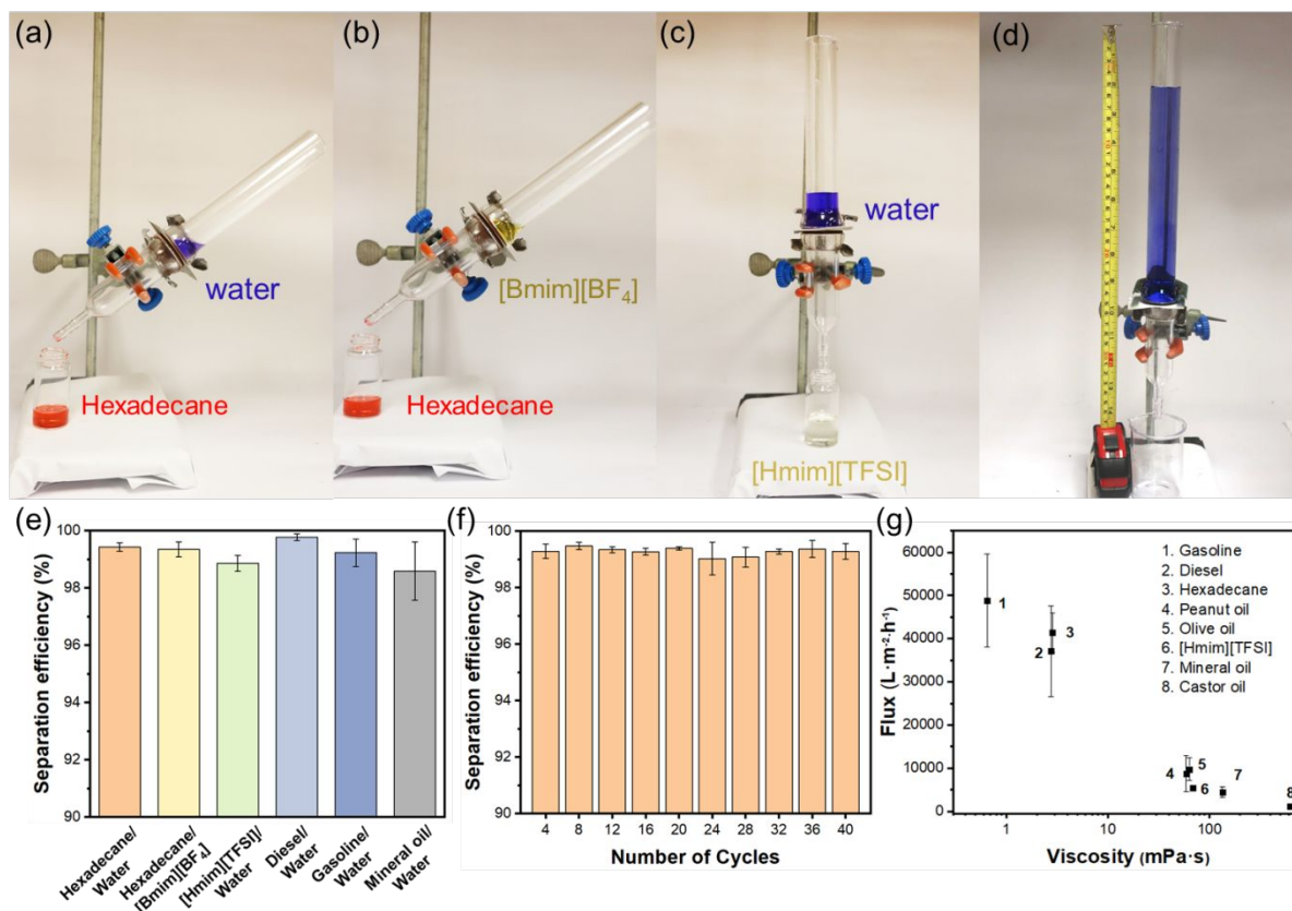
Figure 4. Separation of (a) water/hexadecane, (b) [Bmim][BF 4 ]/hexadecane, and (c) water/[Hmim][TFSI] by T-ZnO/PLMA-40. Water was dyed with Brilliant Blue R and hexadecane was dyed with Oil O Red. (d) Maximum water intrusion pressure of T-ZnO/PLMA-40. (e) Separation efficiency values of T-ZnO/PLMA-40-coated mesh for six pairs of immiscible liquid/liquid mixtures. (f) Separation efficiency for hexadecane/water mixture after varied numbers of cycles. (g) Fluxes of low-surface-energy liquids permeating the mesh
