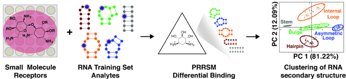
Figure 5: Pattern recognition of RNA by small molecules (PRRSM). An array of small molecule receptors is titrated with RNA secondary structure analytes. Utilizing the small molecule differential binding and an unbiased statistical method allows for clustering based on the RNA structural motifs. Reprinted with permission from Ref. 19. Copyright 2019 American Chemical Society.
