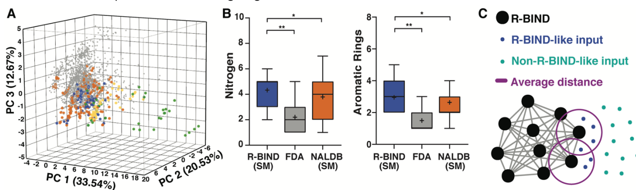
Figure 4. RNA-targeted Bioactive Ligand Database (R-BIND) reveals distinct properties of RNA-targeted small molecules. A. Principle component analysis of R-BIND small molecules (blue), nucleic acid ligand database (NALDB) RNA-binding small molecules (orange), FDA-approved drugs (gray), R-BIND multivalent ligands (green), NALDB multivalent ligands (yellow) based on 20 cheminformatic parameters showing that R-BIND small molecules represent a subset of traditional medicinal chemistry (FDA) space. B. Box-whisker plots of representative parameters showing structural differences between RNA-targeted bioactives (R-BIND SM), protein-targeted bioactives (FDA), and general RNA ligands (NALDB). Panel A,B reproduced from Ref. 35 with permission from John Wiley and Sons. C. Schematic of nearest neighbor analysis where the distance between R-BIND small molecules (black) and input ligands is measured using cheminformatic parameters. The distance between each R-BIND small molecule and its nearest neighbor is averaged (purple) and "R-BIND like ligands" (blue) are defined as those within the average distance to at least one R-BIND ligand. Reprinted with permission from Ref. 36. Copyright 2019 American Chemical Society.
