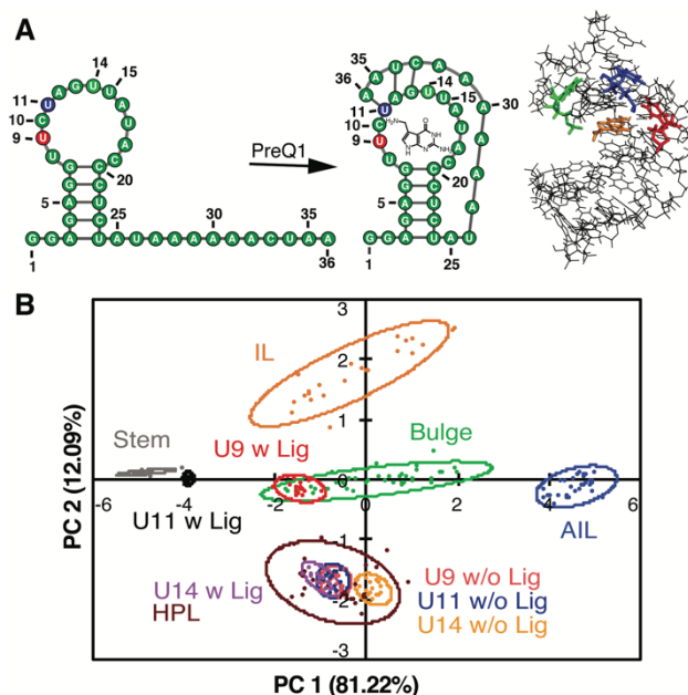
Figure 7. PRRSM classifies apo and bound secondary structures in prequeuosine-1 (PreQ1) riboswitch. A. Left: PreQ1 riboswitch secondary structure in the unbound and bound state. Right: Bound structure of PreQ1 (PDB 2L1V) with highlighted sites of BFU fluorophore insertion (U9-red, U11-blue, U14-green) and PreQ1 ligand (orange). B. PCA plot of the U9, U11, and U14 modified RNA in the absence (w/o Lig) and presence (w Lig) of PreQ1 ligand. All constructs were predicted to be the correct structure in both the unbound and bound states under standard conditions (10 mM NaH 2 PO 4 , 25 mM NaCl, 4 mM MgCl 2 , 0.5 mM EDTA, pH 7.3 at 25 °C. Reprinted with permission from Ref. 112. Copyright 2019 American Chemical Society.
