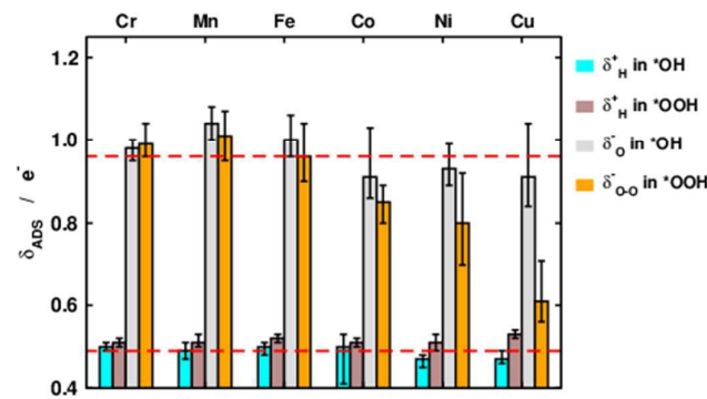
Fig. 4 Excess charge ( \delta^- ) or lack of charge ( \delta^+ ) on H and, O, and O-O in *OH and *OOH. While the charges of H in *OH (light blue), H in *OOH (brown), and O in *OH (gray) are relatively constant for the different metal centers, that of O-O in *OOH (orange) undergoes large changes as the metal ion goes from Cr to Cu. The red dashed lines correspond to the average values of O and H in *OH. Error bars are provided to show the effect of the ring ligands.
