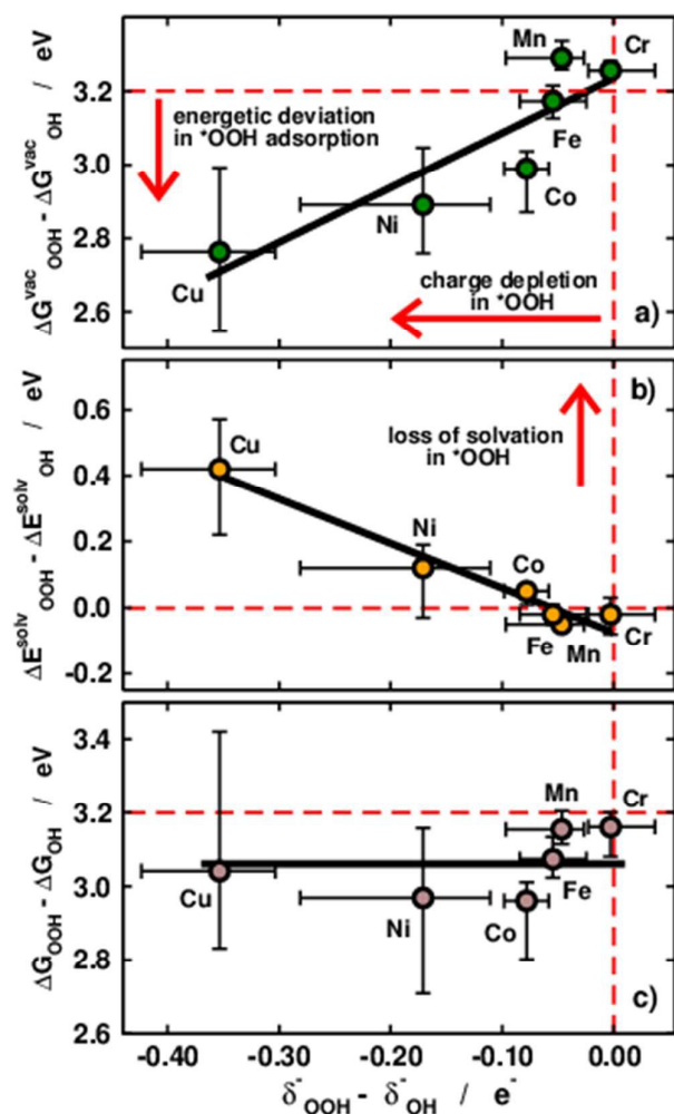
Fig. 5 Covalence effects on *OH and *OOH adsorption. a) Differences in the adsorption energies of *OOH and *OH in vacuum vs the differences in their electronic charges. b) Differences in solvation energies vs differences in electronic charges. In a) and b) the deviations from the ideality grow in opposite directions when going from Cr to Cu, so that the differences in solvated adsorption energies in c) are nearly constant ( \sim 3.1 eV). The dashed lines in a)-c) mark the ideal situation in which *OOH and *OH have identical charges and solvation energies and their energetic separation is 3.2 eV.
