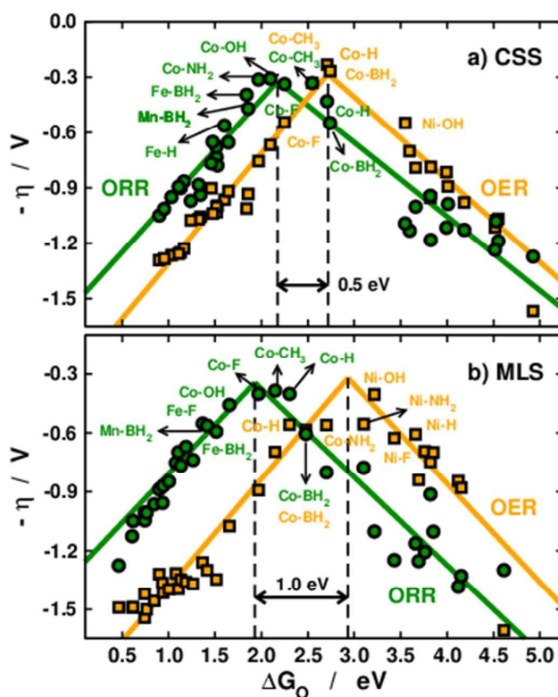
Fig. 6 Volcano-type activity plot for the ORR (green) and the OER (orange). The overpotential ( \eta ) is plotted against the adsorption energies of *O, see section S2 in the ESI. a) Using a constant-shift solvation correction (CSS) from ref. 11, 26 b) Using the metal- and ligand-dependent solvation corrections (MLS) calculated in this study. The black dashed lines mark the top of the OER and ORR volcanoes and show that different solvation treatments lead to different activity predictions.
