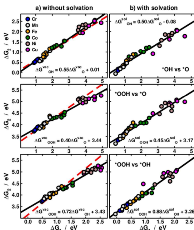
Fig. 3 Scaling relations between the adsorption energies of *O, *OH and *OOH. a) In vacuum, b) solvated. In each panel linear fits (black) and their equations are provided. Top: *OH vs *O; middle: *OOH vs *O; bottom: *OOH vs *OH. The red dashed lines in a) are from ref. 11 and show that while \Delta G_O^{vac} and \Delta G_{OH}^{vac} behave normally (top), \Delta G_{OOH}^{vac} (middle and bottom) causes large deviations in scaling relations. In b) solvation restores the scaling relations broken in vacuum by making the slopes approach the ideal values of 0.5 and 1.
