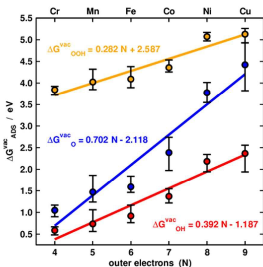
Fig. 2 Adsorption-energy trends of *O (blue), *OH (red) and *OOH (orange) in vacuum for metal centers from Cr to Cu as a function of their number of outer electrons ( N ). The points are the average adsorption energies and the error bars show the energetic effect of the ligands in Fig. 1.
