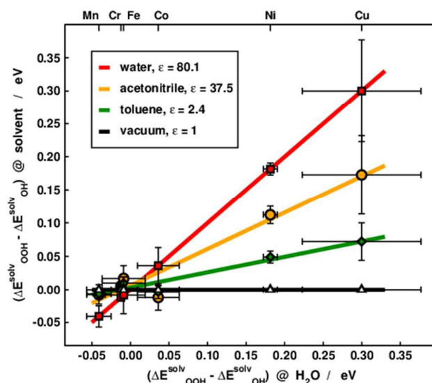
Fig. 7 Comparison between the loss of solvation of ^*OOH with respect to ^*OH in various solvents for porphyrins with -H and -F ligands. Data for water (red), acetonitrile (orange), toluene (green) and vacuum (black), where there is no solvation, are plotted as a function of those of water. Although the solvation losses are small for Cr, Mn, Fe and Co, they are substantial for Ni and Cu and depend on the solvent's dielectric constant. Solvents with small \epsilon such as toluene avoid the restoration of scaling relations broken in vacuum via high covalence.
