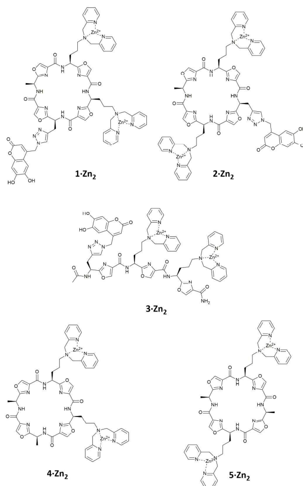
Figure 1: Structures of peptide-based receptors 1–3·Zn 2 , and the previously reported 4–5·Zn 2
