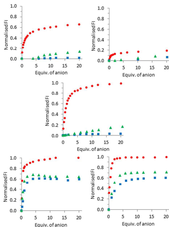
Fig 3. Changes in the fluorescence emission intensity of 1 (top left), 2 (top right), 3 (middle), 4 (bottom left) and 5 (bottom right) at 480 nm upon addition of PPI (●), ATP (▲), and ADP (■) in HEPES buffer (5 mM, 145 mM NaCl, pH 7.4) at 25 °C.
