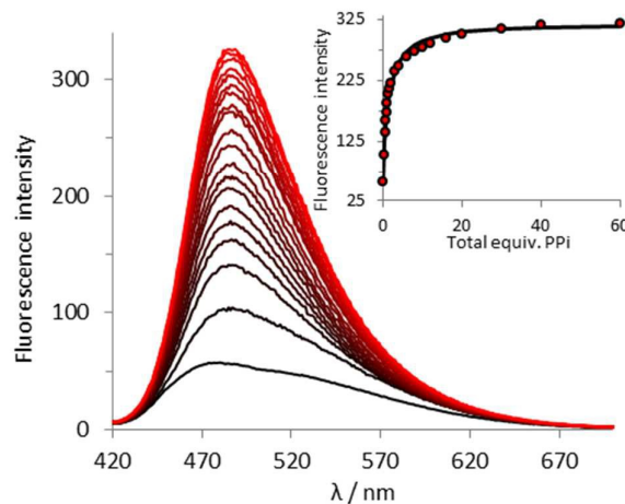
Fig 4 Fluorescence emission spectra of 1 · Zn 2 (5 μM) in response to PPI (0–300 μM) in HEPES (5 mM, 145 mM NaCl, pH 7.4) at 25 °C. λ ex = 390 nm, slits = 5 nm/5 nm.
