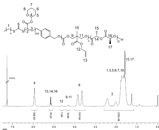
Figure 1. ^1\text{H} NMR spectrum (400 MHz, \text{CDCl}_3 ) of PLLA- b -PMAC- b -PTHPA triblock copolymer, 4 .
