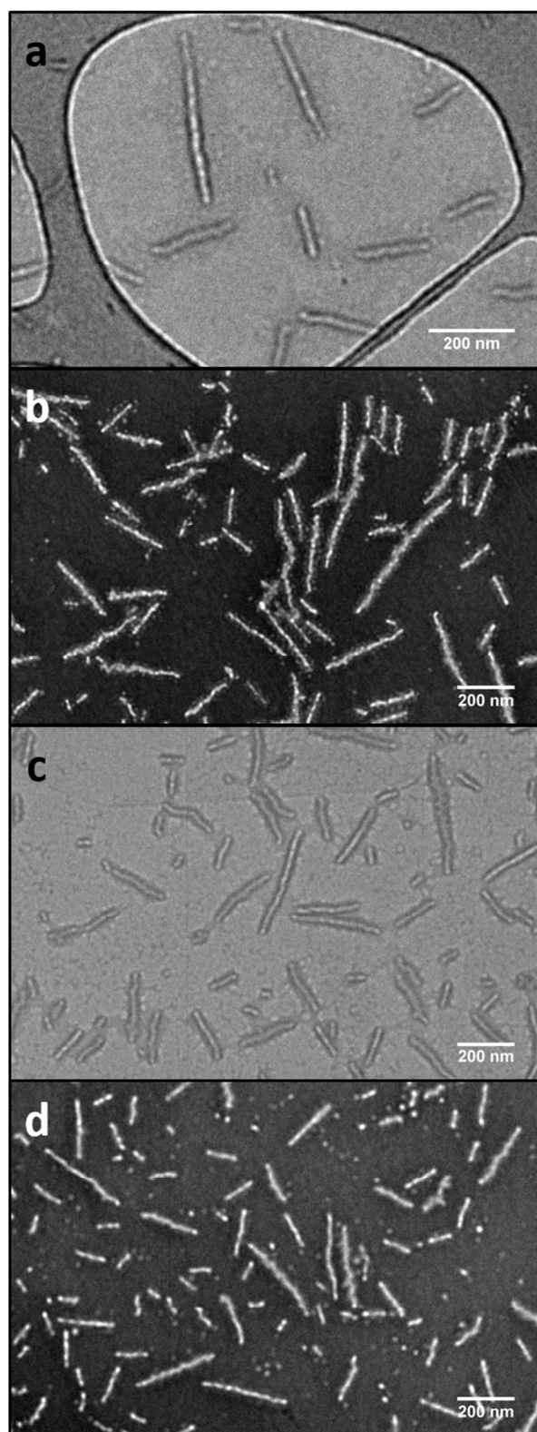
Figure 3 TEM images showing the PLLA- b -PMAC- b -PAA cylindrical micelles before (a and b) and after functionalization with benzyl mercaptan (c and d). a and c, on graphene oxide grid 49 ; b and d, with negative staining using phosphotungstic acid (PTA). Scale bar = 200 nm.
