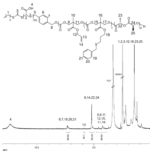
Figure 4. ^1\text{H} NMR spectrum (500 MHz, d_6 -DMSO) of benzyl mercaptan functionalized PLLA- b -PMAC- b -PAA cylindrical micelles.
