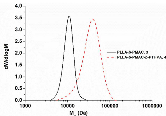
Figure 2. SEC chromatograms ( \text{CHCl}_3 with 0.5% TEA as eluent, RI detection) of PLLA- b -PMAC diblock copolymer, 3 and PLLA- b -PMAC- b -PTHPA triblock copolymer, 4 .
