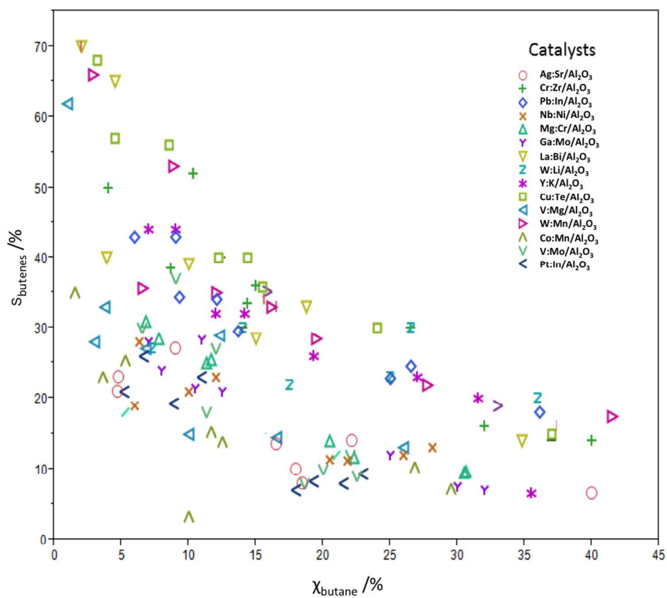
Figure 1. Summary plot showing the percentage total selectivity for butenes vs. the percentage conversion of n-butane for catalysts 1–15 under condition sets A–H.
