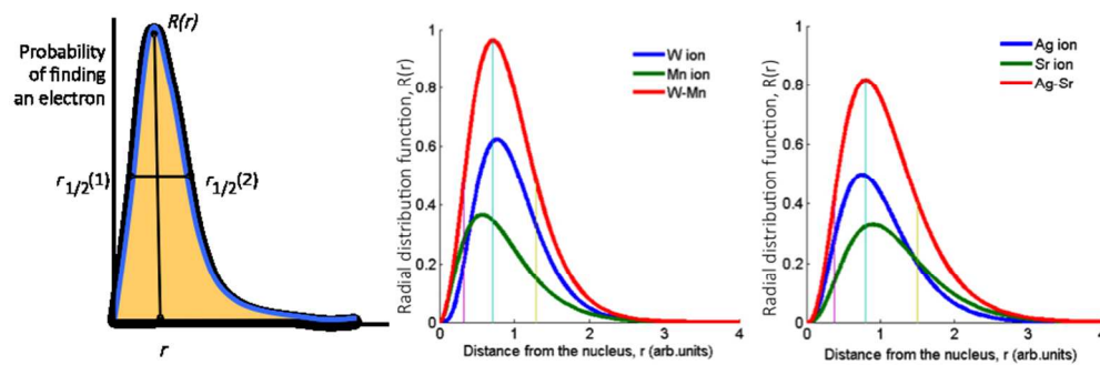
Figure 2. Graphs showing a typical radial distribution function (RDF) based on the Slater-type orbitals used for deriving the four descriptors for (mixed) oxides (left), and examples of these orbitals for AgOx:SrOx/Al 2 O 3 (catalyst 1) and WOx:MnOx/Al 2 O 3 (catalyst 12).
