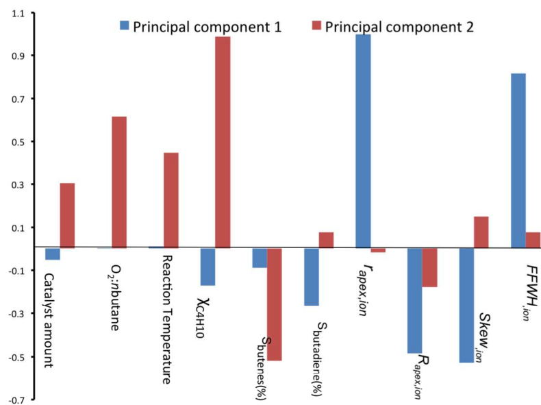
Figure 4. Bar chart showing the loading coefficients of each sample on the two first principal components.
