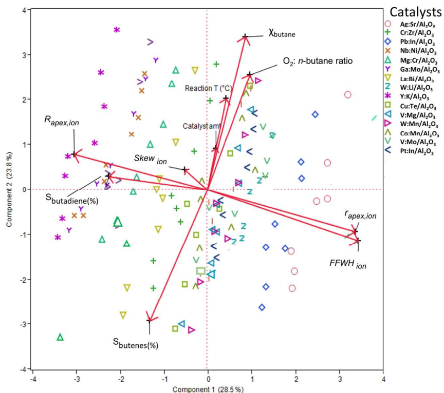
Figure 3. Biplot representation following a principal component analysis (PCA) of the experimental results, showing the distribution of the conversion and selectivity of catalysts 1–15 running under reaction conditions A–H in the space of the two first principal components. Each symbol represents one catalyst under one set of reaction conditions. The arrows indicate the direction and magnitude of the descriptors and the figures of merit. For example, the fact that the \text{FFWH}_{\text{ion}} arrow is opposite to S_{\text{butadiene}}(\%) means that oxides with a higher \text{FFWH}_{\text{ion}} value will give less butadiene. Similarly (and unsurprisingly) the conversion of butane is strongly correlated with the oxygen:butane ratio.
