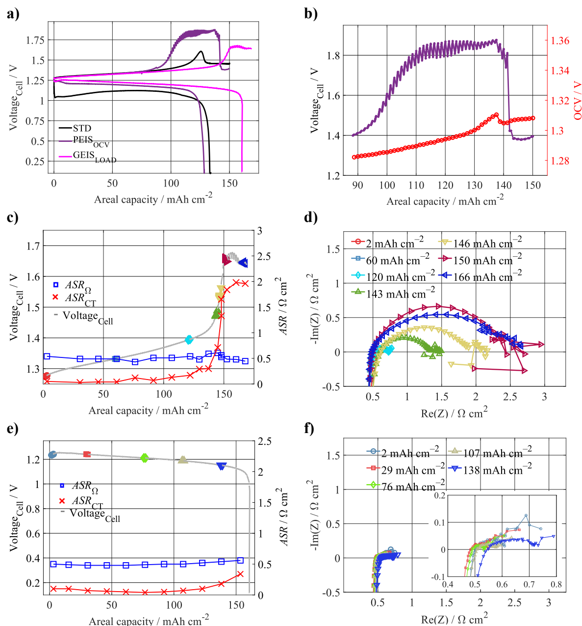
Figure 6: a) U-Q_{\text{areal}} dependence of a charge-discharge cycle for different characterization techniques STD, \text{PEIS}_{\text{OCV}} and \text{GEIS}_{\text{LOAD}} for ZIHFB with omitted zinc ions in posolyte (besides STD). b) \text{OCV}_{\text{Cell}} dependence on Q_{\text{areal}} during \text{PEIS}_{\text{OCV}} characterization. c) U-Q_{\text{areal}} dependence during \text{GEIS}_{\text{LOAD}} characterization with evaluated \text{ASR}_{\text{CT}} and \text{ASR}_{\text{O}} , colours used in the voltage cell evolution are linked to d) where EIS spectra are displayed with colour for corresponding Q_{\text{areal}} . Figures e) and f) represents the same as c) and d) , but for battery discharge. Experimental conditions: Std. negolyte composition, \text{ZnI}_2 omitted from posolyte (besides STD); Both electrolytes' volumes 0.07 \text{ dm}^3 .
