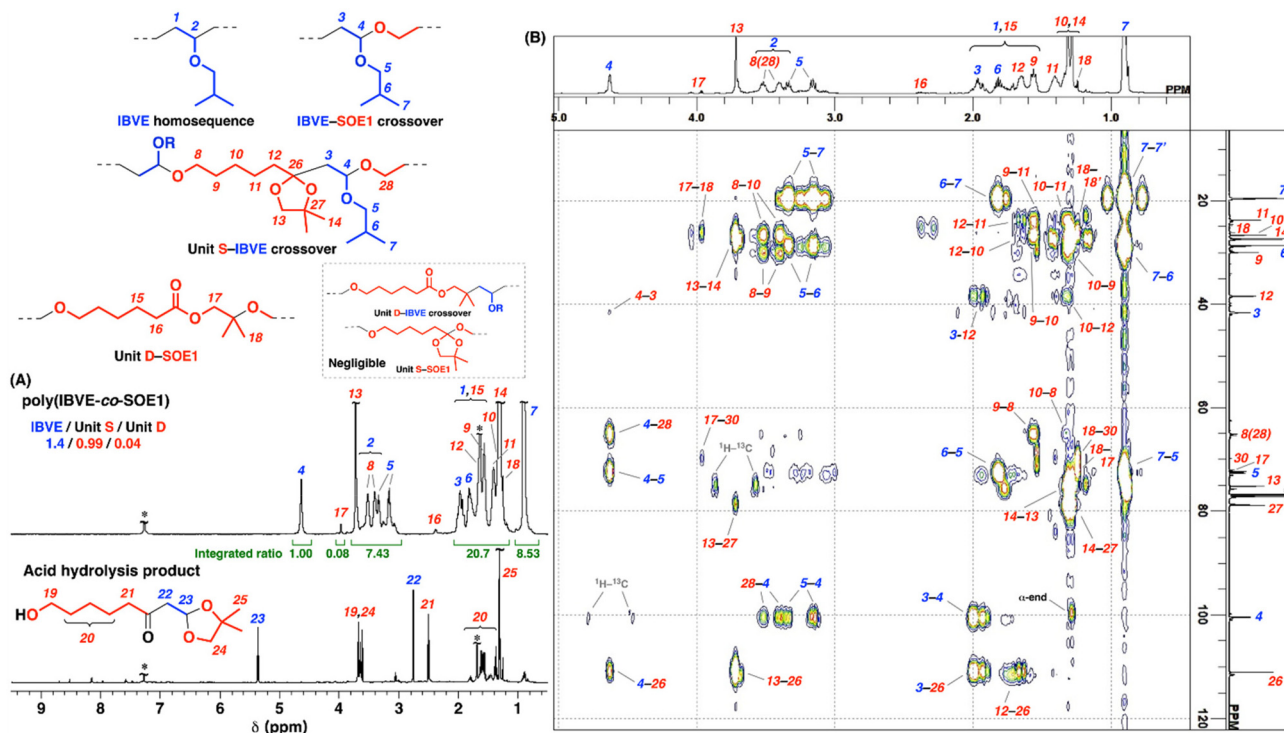
Fig. 2 (A) 1 H NMR spectra of poly(IBVE-co-SOE1) (upper; entry 5 in Table 1; after purification by reprecipitation in methanol, a pink curve in Figure 1B) and acid hydrolysis product (lower). (B) 1 H- 13 C HMBC NMR spectrum of poly(IBVE-co-SOE1) (entry 9 in Table 1; a limited region of the spectrum is shown; see Fig. S9 for a wider region). See the footnote of Table 1 for the polymerization conditions. In CDCl 3 at 30 °C. *CHCl 3 or water.
