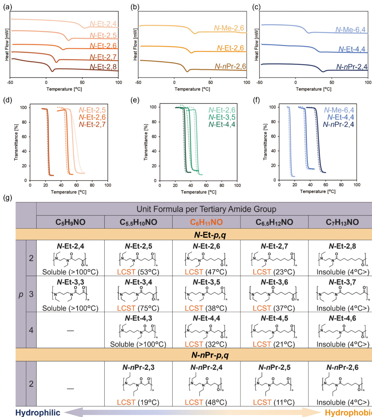
Fig. 2 Thermal property and aqueous solubility of N -alkylated nylons. DSC second heating thermogram ( 10\text{ }^\circ\text{C min}^{-1} ) of (a) N -Et-2, q ( q = 4–8), (b) N -R-2,6 (R = Me, Et, and n Pr), and (c) N -alkylated nylons with C_6H_{11}NO ( N -Me-6,4, N -Et-4,4, N - n Pr-2,4). Transmittance change at 800 nm of (d) N -Et-2, q ( q = 5–7), (e) N -Et- p,q ( p,q = 2,6, 3,5, 4,4), and (f) N -alkylated nylons with C_6H_{11}NO ( N -Me-6,4, N -Et-4,4, N - n Pr-2,4) in H_2O ( 10\text{ mg mL}^{-1} ) by the temperature changes (scan rate: 1.5\text{ }^\circ\text{C min}^{-1} ); the solid and dotted lines represent the heating and cooling processes, respectively. (g) Summary of the solubility of a series of N -alkylated nylons in H_2O ( 10\text{ mg mL}^{-1} ). The vertical axis represents the methylene carbon numbers of the diamine moiety ( p ), and the horizontal axis represents the unit formula per tertiary amide group. Each entry is classified as soluble, LCST-type phase separation, or insoluble; for LCST-type polymers, the cloud point ( ^\circ\text{C} ) at 10\text{ mg mL}^{-1} is given in parentheses.
