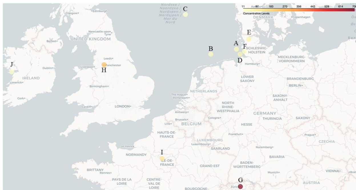
Figure 6 Atmospheric concentrations of 8:2 FTOH (pg/m 3 ) in selected regions in Europe, as reported in prior studies 61,83–87 . Measurements in the following locations are reported: A: German Bight, B: Heligoland, C: West Frisian coast, D: Cuxhaven, E: Schleswig-Holstein, F: Büsum, G: Zurich, H: Manchester, I: Paris, J: Mace Head.
