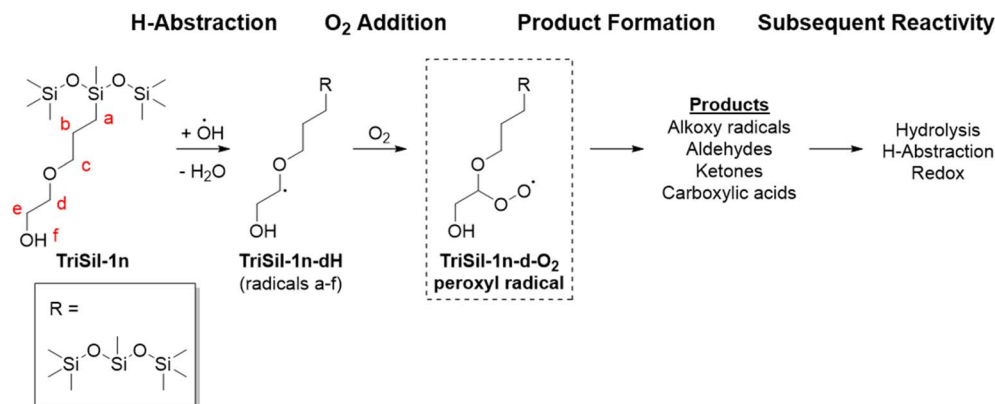
Fig. 4 TriSiI-1n degradation reaction channel for hydroxyl radical induced degradation via H-abstraction. See Scheme S1† for a proposed reaction diagram for TriSiI-1n-d-O 2 peroxy radical.
