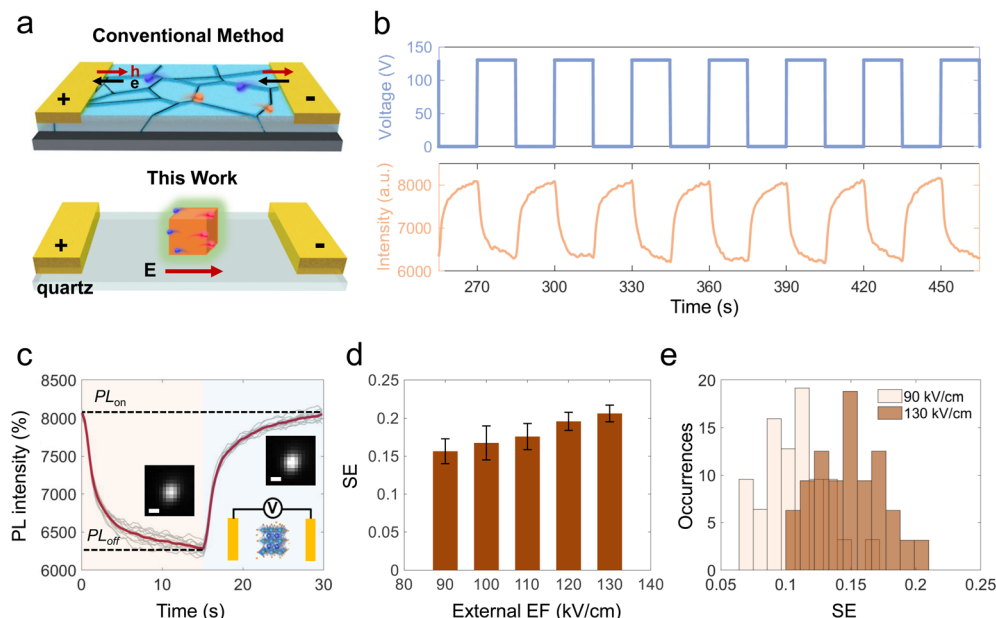
Fig. 1 The optical measurements of MAPbBr 3 under an external electric field. (a) The schematic of a classical contact perovskite device (top) and the electric field-induced non-contact perovskite device in this work (bottom). (b) The evolution of PL intensity with time under external electric field control. (c) The evolution of the PL intensity for a 10-cycle superposition (grey line) and the average curve (red line). The inset is the raw image of individual MAPbBr 3 particles with/without the external electric field. (d) The switching efficiency of an individual particle with different external electric fields in 10 cycles. (e) The histogram of switching efficiency for 43 particles at different external electric fields.
