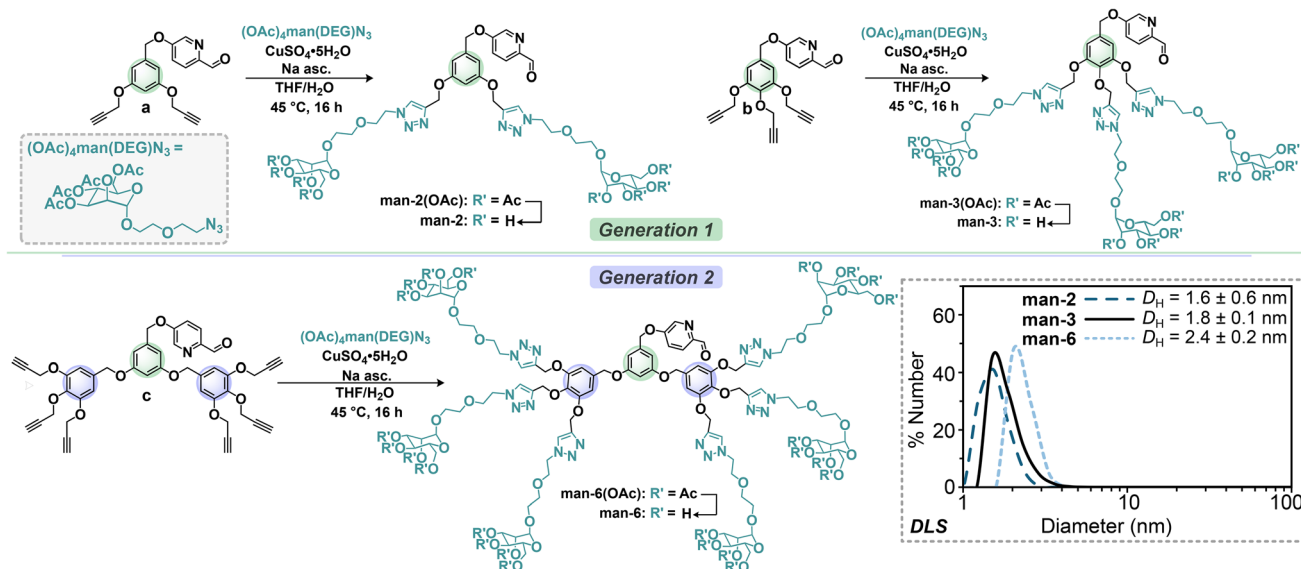
Fig. 2 Synthetic schemes for the preparation of dendritic subcomponents man-2 , man-3 , and man-6 from a , b , and c precursors, respectively, with corresponding DLS data (bottom right, measured in \text{H}_2\text{O} , 1 mM).
