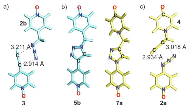
Fig. 3 (a) Arrangement of the reacting substrates in the energy-minimized structures of: (a) the (\mathbf{2b}\cdot\mathbf{3})\cdot\mathbf{1} ternary hetero-complex and (c) the (\mathbf{2a}\cdot\mathbf{4})\cdot\mathbf{1} ternary hetero-complex. The \text{N}_{\text{azide}}-\text{C}_{\text{acetylide}} distances are shown. (b) Energy-minimized structures of the 1,4-triazole isomers 5b (light-blue) and 7a (light-yellow) in the complexes \mathbf{5b}\cdot\mathbf{1} and \mathbf{7a}\cdot\mathbf{1} . For clarity the structure of cage 1 is not shown in the figures.
