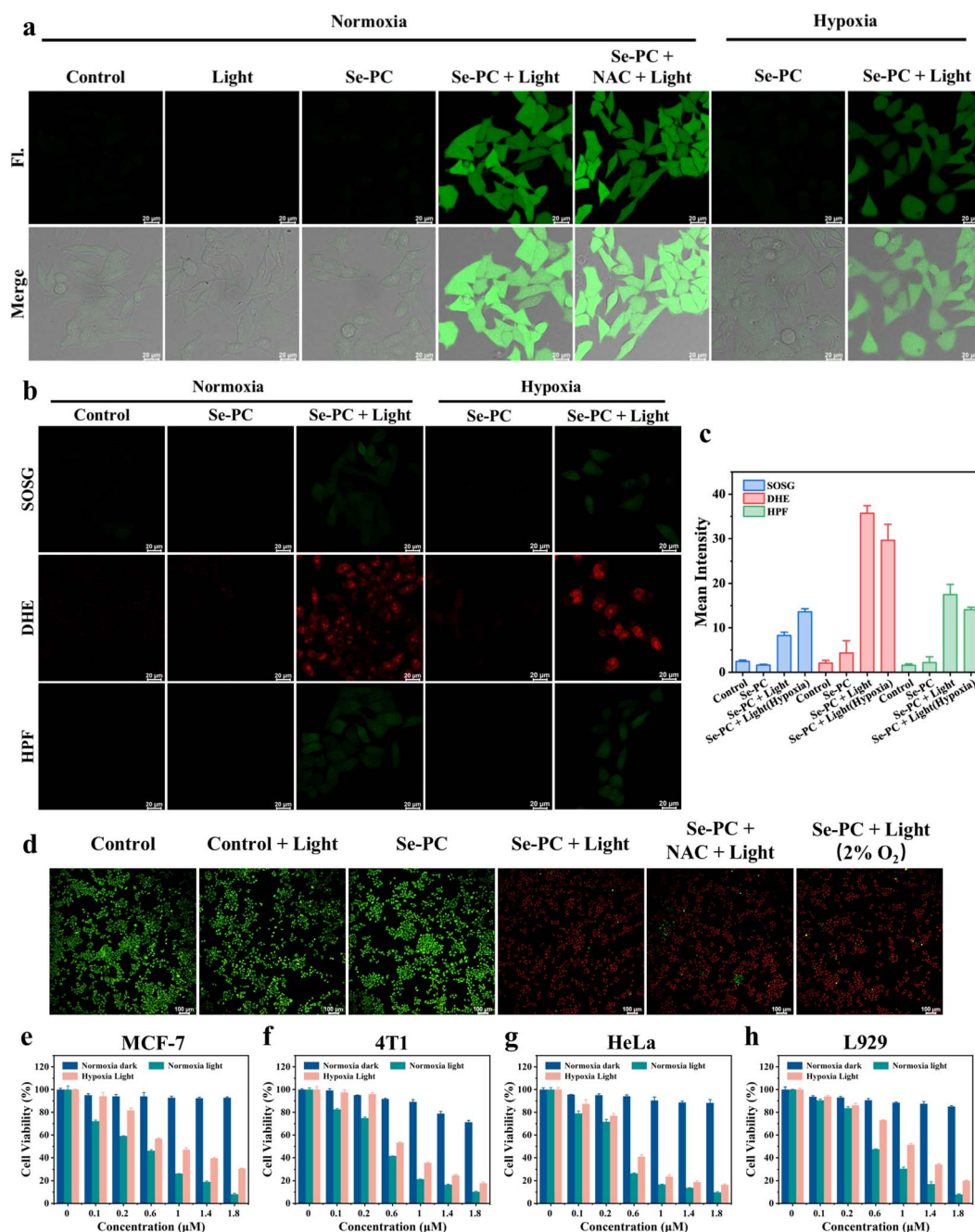
Fig. 3 Intracellular ROS production induced by Se-PC (1 μM) in MCF-7 cells under different conditions, monitored using specific ROS indicators. (a) The total ROS indicator DCFH-DA. (b) The ^1\text{O}_2 indicator SOSG, the \text{O}_2^{\cdot-} indicator DHE and the \cdot\text{OH} indicator HPF. (c) Quantitative analysis corresponding to (a) and (b). Scale bar: 20 μm. (d) Confocal images of MCF-7 cells co-stained with the calcium-AM/PI test kit after different treatments. Scale bar: 100 μm. Cell viability of (e) MCF-7, (f) 4T1, (g) HeLa and (h) L929 cells co-incubated with different concentrations of Se-PC after different treatments.
