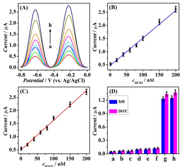
Fig. 6 (A) DPV curves to HClO and H 2 O 2 with different concentrations (from (a) to (h): 1, 20, 40, 60, 80, 100, 150, and 200 nM). The linear fit of (B) I_{DOX} versus c_{HClO} and (C) I_{MB} versus c_{H_2O_2} . (D) Selectivity of the sensing system for HClO (80 nM) and H 2 O 2 (80 nM) against other interferents of 800 nM: (a) blank, (b) NaNO 2 , (c) UA, (d) AA, (e) NaNO 3 , (f) GSH, (g) HClO and H 2 O 2 , and (h) the mixture of HClO, H 2 O 2 , and interferents. Error bar: SD and n = 3 .
