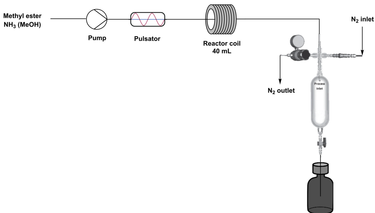
Fig. 6 Schematic overview of continuous flow setup (mini CØPE reactor). *This system was constructed as a down-scaled model of the CØPE reactor of Ajinomoto Omnicheem, Belgium.
