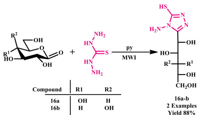
Scheme 10 Microwave-assisted synthetic protocol for 4-amino 3-(D-glucopentitol-1-yl)-5-mercapto-1,2,4-triazole (16a and 16b). 45
