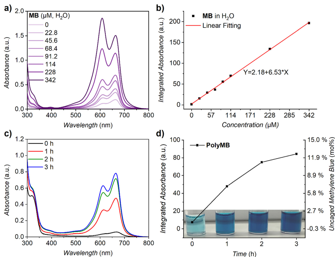
Fig. 5 Red light photoinduced uncaging kinetics of PolyMB (57 \mu\text{M} in H 2 O). (a) UV-vis spectra of different concentrations of methylene blue in water; (b) linear fitting of integrated UV absorbance of methylene blue ( i.e. \int_{420 \text{ nm}}^{800 \text{ nm}} absorbance) as a function of different concentrations of methylene blue solution in water; (c) UV-vis spectra of PolyMB (57 \mu\text{M} ) after different irradiation times ( \lambda_{\text{max}} = 630 \text{ nm} , 18 \text{ mW cm}^{-2} ); (d) integrated UV absorbance ( i.e. \int_{420 \text{ nm}}^{800 \text{ nm}} absorbance) of photoirradiated PolyMB at different time points and the amount of uncaged methylene blue (mol%) calculated based on the linear fitting in (b).
