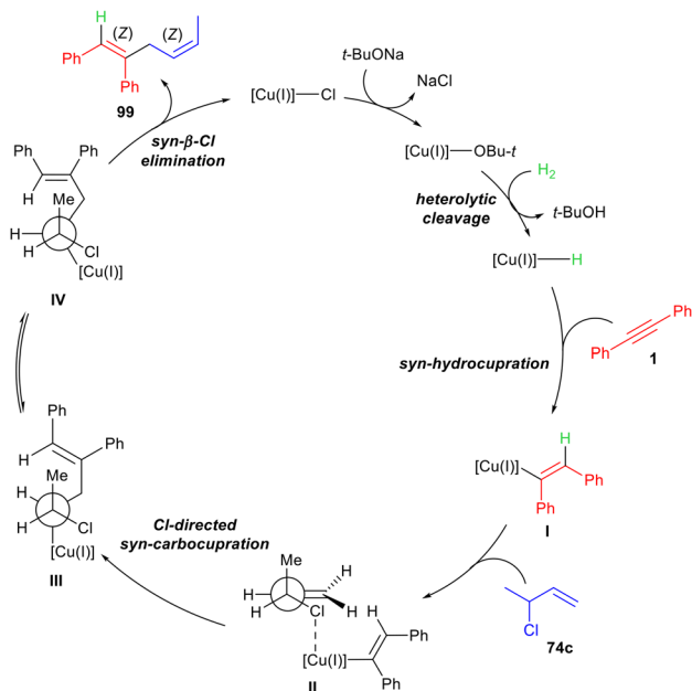
Scheme 41 Plausible reaction mechanism for the \text{Cu}(\text{I}) -catalysed C–C coupling.
