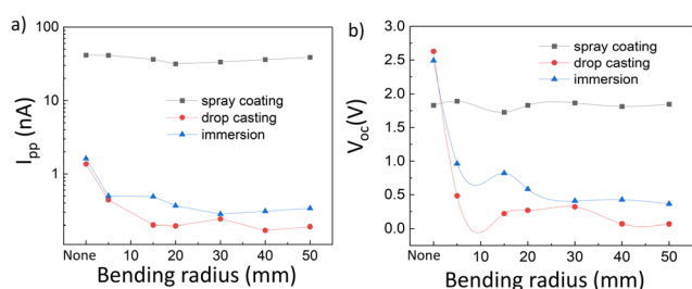
Fig. 5 Summary of measurements after bending tests with varying bending radii, ranging from no bending to 50 mm, for the samples produced by the three different deposition methods. Panel (a) shows the peak-to-peak short-circuit current ( I_{pp} ) and panel (b) shows the open-circuit voltage. The counter triboelectric layer is PVC for drop casting and immersion and nylon for spray coating.
