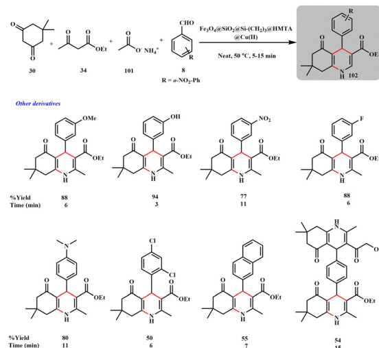
Scheme 46 Catalytic synthesis of hexahydroquinoline derivatives using an Fe 3 O 4 @SiO 2 @Si-(CH 2 ) 2 @HMAT@Cu nanocomposite (Salem et al. ).
