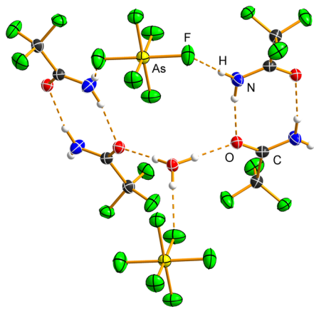
Fig. 5 R 6 6 (20) hydrogen-bonded cluster in the crystal structure of the H 3 O[AsF 6 ] 2 CF 3 CONH 2 salt cocrystal. Hydrogen bonds are shown by dashed orange lines. Displacement ellipsoids are drawn at the 50% probability level, and hydrogen atoms are represented as spheres of arbitrary radius.
