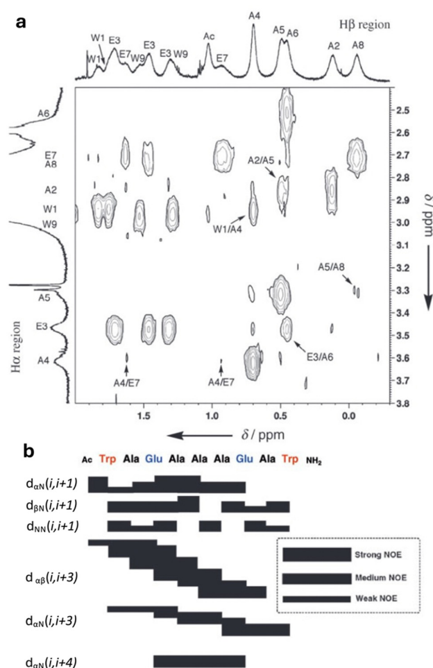
Fig. 3 (a) Selected NOESY spectrum for the assignment of bound peptide (600 MHz, \text{H}_2\text{O}/\text{D}_2\text{O} = 9/1 , 27 °C, 100 mM phosphate buffer, pH 6.8), [\text{2}] = 10 \text{ mM} , [\text{peptide}] = 2.5 \text{ mM} . Proton resonances labelled with single letter amino acid code and residue number corresponding to peptide in Fig. 2a; (b) NOE correlations for peptide 2 . Reproduced with permission from ref. 16.
