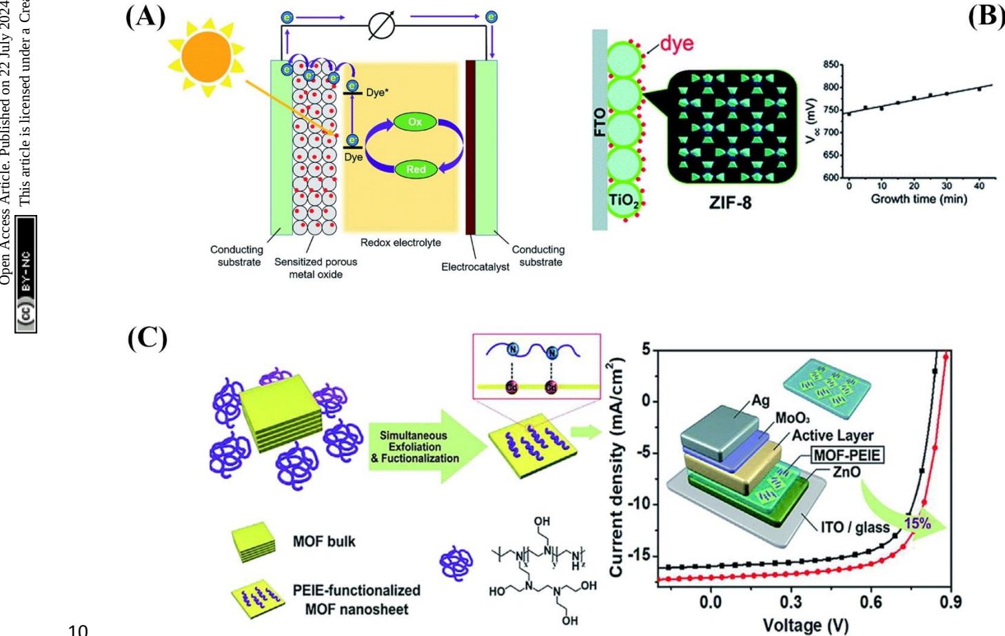
Fig. 4 (a) Schematic representation of typical dye-sensitized solar cells. (b) The use of MOFs for the photoanodes in DSSCs as the blocking layer [72]. (c) Schematic illustration of the preparation of 2D MOF nanosheets and their modified electron-extraction layer for photovoltaic devices [78].
