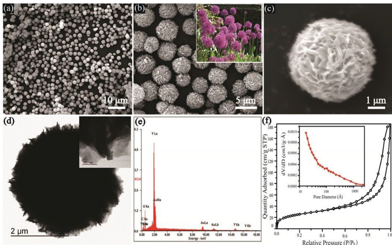
Fig 1. SEM and TEM images of as-prepared Y-MOFs samples at 120 °C for 24 h: (a–c) low- and high-magnification SEM images (inset in (b) is the photo of allium giganteum) [26]; (d) low- and high-magnification TEM images; (e) EDX spectrum [26]; (f) Nitrogen adsorption/desorption isotherms of Y-MOFs: 10%Eu 3+ (inset is pore size distribution) [31].
