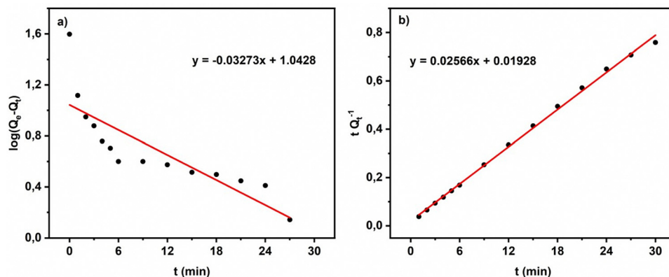
Fig. 9 Kinetic orders for the adsorption process of MG by ACCu1: (a) pseudo-first order, (b) pseudo-second-order.
