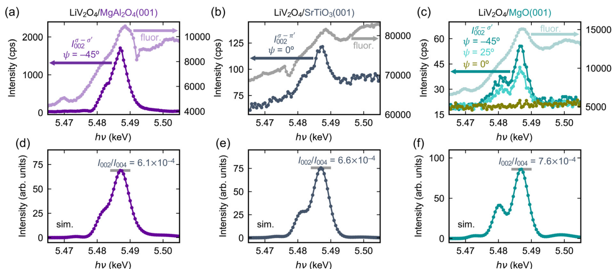
Fig. 4 (a)–(c) Left axes: Anomalous photon energy ( h\nu ) dependence of the resonant forbidden ( 002 ) reflections in \text{LiV}_2\text{O}_4 thin films on various substrates. Each data point represents the maximum ( 002 ) intensity (cps) at the given energy. For (a) and (c), the polarization channel is \sigma - \sigma' and the azimuthal angle is \psi = -45^\circ . For (b), the signal is clearer in the \sigma - \pi' channel at \psi = 0^\circ due to some background in the \sigma - \sigma' channel. Right axes: Fluorescence (fluor.) spectra shown for reference, with intensity reported in cps. (d)–(f) Simulated REXS ( 002 ) spectra using FDMNES. The ratio of the maximum intensities of the ( 002 ) and ( 004 ) reflections as predicted by the simulations (sim.) are labeled with horizontal gray bars.
