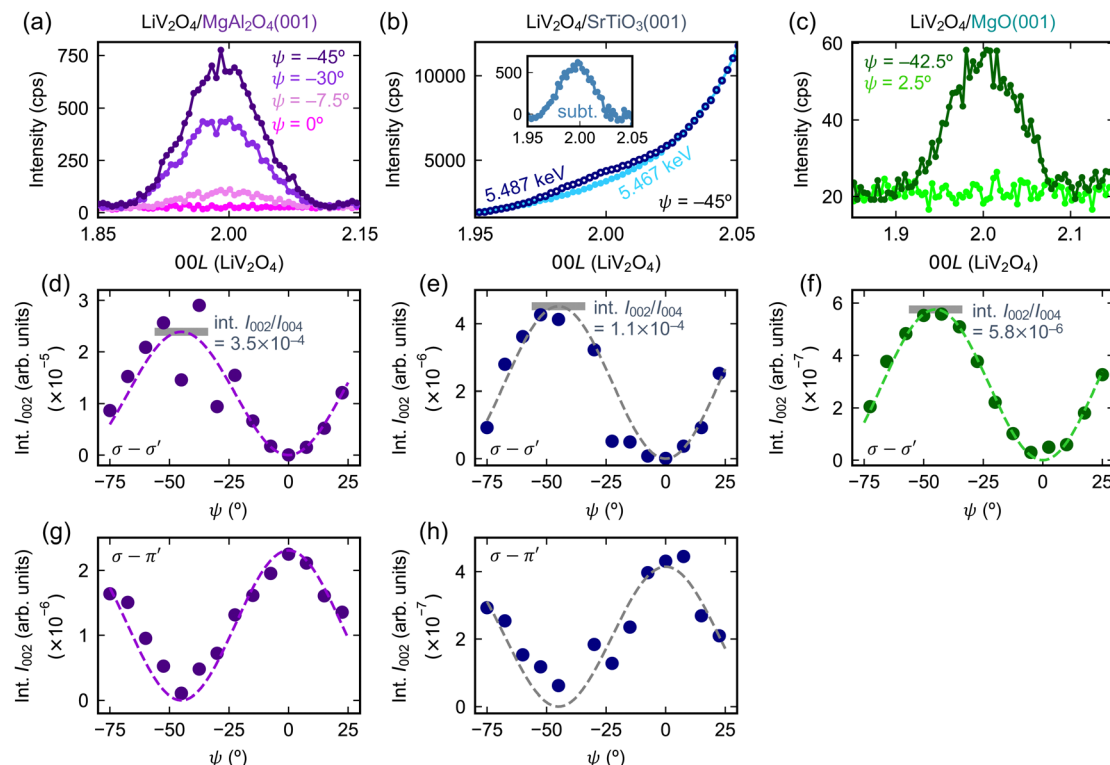
Fig. 3 (a)–(c) Resonant forbidden ( 002 ) reflections at the V K edge in \text{LiV}_2\text{O}_4 thin films on various substrates. The photon energy used is 5.487 keV unless otherwise noted, and the polarization channel is \sigma - \sigma' . The intensity is reported in counts per second (cps). In the case of \text{LiV}_2\text{O}_4/\text{SrTiO}_3 (b), the \text{LiV}_2\text{O}_4(002) reflection is more difficult to observe, because of a large background tail from a nearby substrate reflection, \text{SrTiO}_3(001) . The inset of (b) has the same axes as the main panel and shows the subtraction (subt.) of the data in the main panel. (d)–(h) Azimuthal dependence of the integrated intensity (int. I ) of the resonant forbidden ( 002 ) reflections in the \sigma - \sigma' and \sigma - \pi' channels. The dotted lines are fits to eqn (4) in (d)–(f) and eqn (5) in (g) and (h). The horizontal gray bars in (d)–(f) label the maxima extracted from the fits, normalized by the intensity of the non-resonant ( 004 ) reflection.
