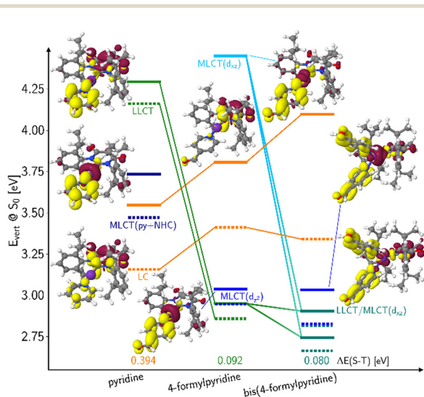
Fig. 1 DFT/MRCI energy level scan of the linear complexes with a pyridine or 4-formylpyridine ligand, respectively, and the bis(4-formylpyridine) complex 3b at the ground-state geometry in dichloromethane solution and assignment of the electronic structures of the excited states. Solid lines represent singlet states, dashed lines triplets. Excitations are characterised by difference density plots (isovalue \pm 0.002 ). A loss of electron density with respect to the electronic ground state is shown in red, a gain in yellow.
