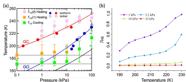
Figure 5. (a) Correlation of the gated CO 2 sorption behaviour with the SCO transition temperatures of framework 1 under variable CO 2 pressure in the temperature range of 160\text{--}260\text{ K} ; (b) HS fraction population ( \gamma_{HS} ) of 1 under variable CO 2 pressure ( P_{CO_2} = 1 to 32\text{ kPa} ) in the temperature range of 190\text{--}230\text{ K} .
