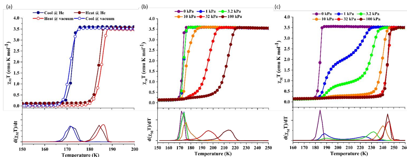
Figure 4. Variation of the magnetic properties of Framework 1 under CO 2 adsorption under H_{dc} = 1\text{ kOe} . (a) magnetic susceptibility plots in the absence of any gas (open circles) and under 100 kPa He gas (filled circles). (b) The CO 2 pressure dependence of the magnetic susceptibility measurements in cooling and (c) heating mode. First derivative plots are displayed at the bottom.
