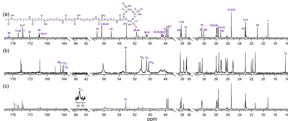
Fig. 3 \{^1\text{H}\}-^{13}\text{C} NMR spectra from solutions ( \text{D}_2\text{O} ) of (a) 3a , (b) \text{Zr(IV)} : \textbf{3a} (0.8 : 1), or (c) \text{Lu(III)} : \textbf{3a} (0.8 : 1).
